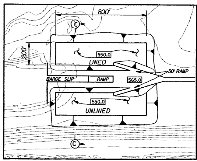
DETAIL - DISPOSAL UNLOADING AREA
