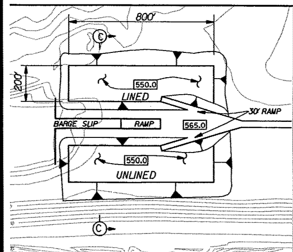
DETAIL - DISPOSAL UNLOADING AREA
