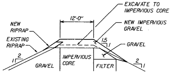
LEVEE RAISE < 2'
