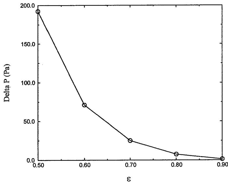
Figure 4. Effect of external void fraction on pressure drop
