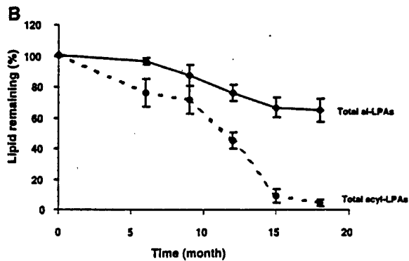
Fig. 1. Alkyl- and alkenyl-lysophosphatidic acids (al-LPAs) in ascites from ovarian cancer patients are more stable than acyl-LPAs. Al-LPAs and acyl-LPAs from ascites samples were extracted and analyzed as described in Materials and Methods. Five ascites samples from patients with ovarian cancer were stored at 4°C under sterile conditions. LPAs from 0.5 ml of ascites were analyzed at the time intervals as indicated. A: Electrospray ionization mass spectrometry (ESI-MS) spectra of LPAs from representative ovarian cancer ascites samples analyzed at 0, 6, 12, and 18 months. B: The stability of LPAs in five ovarian cancer ascites samples.
