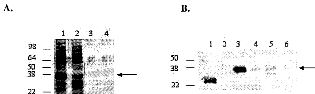
Fig. 3. Enzymatic activity assay using FP-biotin probe.
