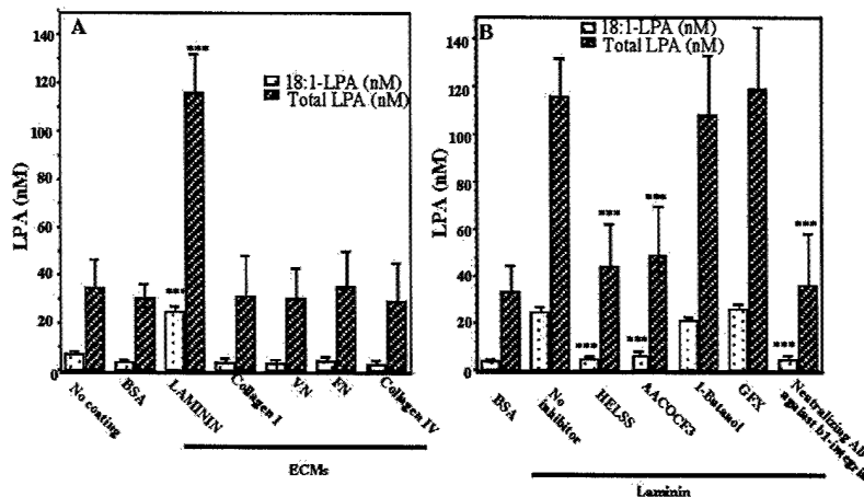
Fig. 7 Laminin-induced LPA production in HL 1 cells. A. 6-well plates were coated with different ECMs (10 \mu g/mL) and blocked with BSA (0.1%). Starved HEY cells ( 5 \times 10^5 - 10^6 /well) were incubated in these wells for 4 hr. Cell supernatant was collected. LPA extraction and analyses were performed as described previously 6 (appendix 1). B. 6-well plates were coated with laminin and blocked with BSA. Starved HEY cells were treated with or without inhibitors or the neutralizing antibody against \beta_1 integrin prior to incubation in the coated wells. LPA production (18:1-LPA and total LPA) was presented as the mean \pm S.D. of three independent experiments. *** = p < 0.001 when compared with controls.
