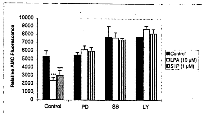
Fig. 8. LPA and S1P reduced paclitaxel-induced caspase-3 activity. HEY cells were pretreated with 30 μM PD98059 (PD), 10 μM SB203580 (SB), or 10 μM LY294002 (LY) for 30 min, then treated with LPA (10 μM) or S1P (1 μM) for 20 min, followed by exposure to paclitaxel (1 μM) for 24 h. Caspase-3 activity was determined by cleavage of the fluorogenic substrate, N -acetyl-Asp-Glu-Val-Asp-amino-4-methylcoumarin. ***, p < 0.001 (Student's t -test).
