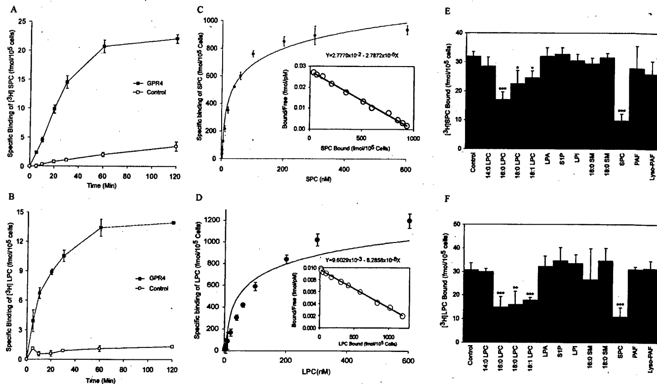
FIG. 4. Binding of SPC and 16:0-LPC to GPR4. A and B, time dependence of specific [ 3 H]SPC and [ 3 H]LPC binding. Cell homogenates (100 \mu l, equivalent to 10 5 cells) from vector or GPR4 stably transfected CHO cells were incubated with [ 3 H]SPC (1 nM) or [ 3 H]16:0-LPC (1 nM) for the indicated times. Specific binding is shown. C and D, saturation isotherm of specific binding of [ 3 H]SPC and [ 3 H]16:0-LPC to GPR4-transfected CHO cells. Cell homogenates (100 \mu l) were incubated with the indicated concentrations of [ 3 H]SPC or [ 3 H]16:0-LPC in the presence or absence of unlabeled SPC (100-fold excess) or unlabeled 16:0-LPC (100-fold excess). Specific binding is presented. E and F, structural specificity of binding of [ 3 H]SPC and [ 3 H]16:0-LPC to GPR4. GPR4-transfected CHO cells were incubated with [ 3 H]SPC (1 nM) or [ 3 H]16:0-LPC (1 nM) in the presence or absence of 100 nM of different unlabeled lipids. Total binding is presented. All binding experiments were performed in triplicate in 96-well plates. Data are mean \pm S.D. from three independent experiments. *, p < 0.05 ; **, p < 0.01 ; ***, p < 0.001 ; as compared with the control (Student's t test).
