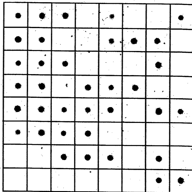
FIG. 1. GPR4 expression in different human tissues. The human RNA Master Blot (CLONTECH) was probed with ^{32}\text{P} -labeled GPR4 ("Experimental Procedures").
