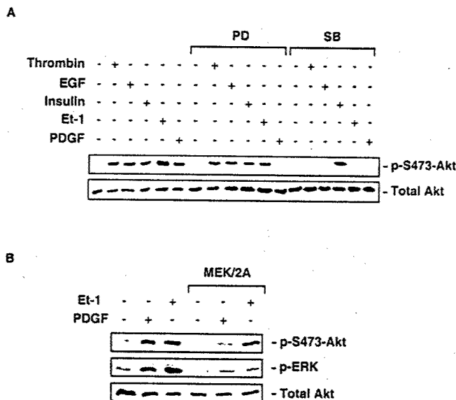
Fig. 5. Stimulus-specific S473 phosphorylation of Akt. Western analyses of HEY cell lysates probed with p-S473-Akt, and then reprobred with p-ERK or total Akt antibodies. A, cells were pretreated with 30 \mu M PD98059 (PD) or 10 \mu M SB203580 (SB) for 30 min followed by treatment with thrombin (1 U/ml), EGF (10 ng/ml), insulin (100 nM), Et-1 (100 nM), or PDGF-BB (10 ng/ml) for 5 min. B, cells transiently transfected with MEK/2A were treated with Et-1 (100 nM) or PDGF-BB (10 ng/ml) for 5 min.
