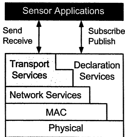
Figure 1-2: Declarative Networking
