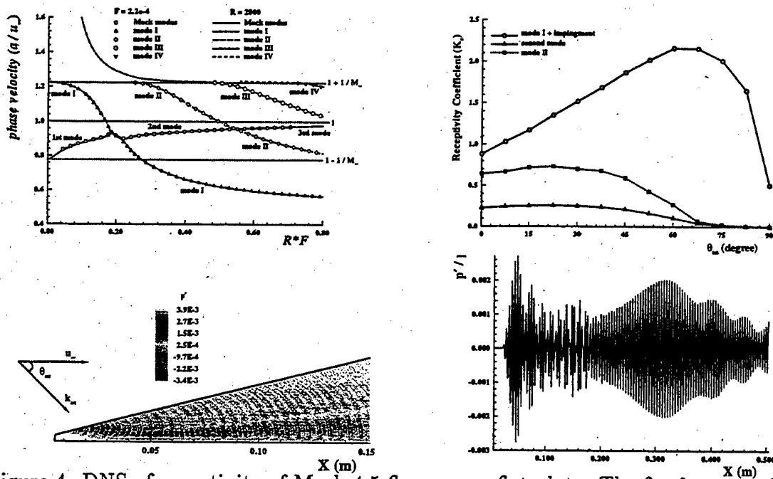
Figure 4: DNS of receptivity of Mach 4.5 flow over a flat plate. The forcing wave is a plane acoustic wave with zero angle ( F = 2.2 \times 10^{-4} ).
