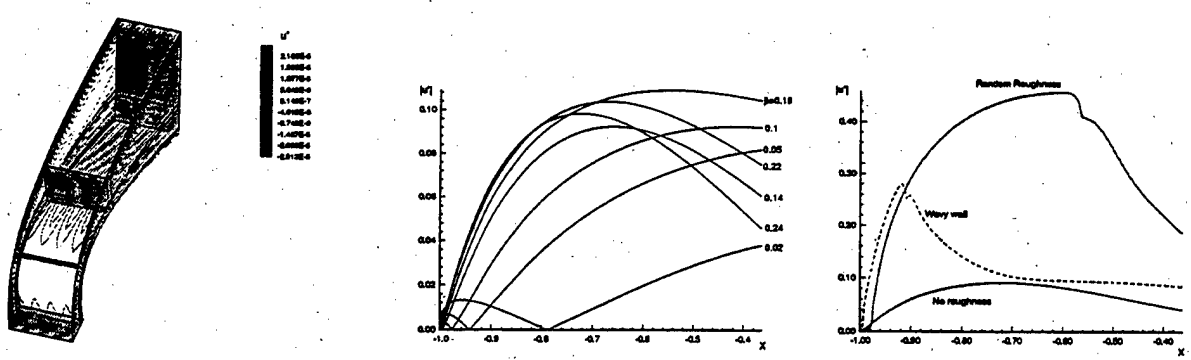
Figure 8: DNS of receptivity and transient growth due to streamwise vorticity waves in a Mach 15 flow over a blunt wedge (with and without surface roughness).
