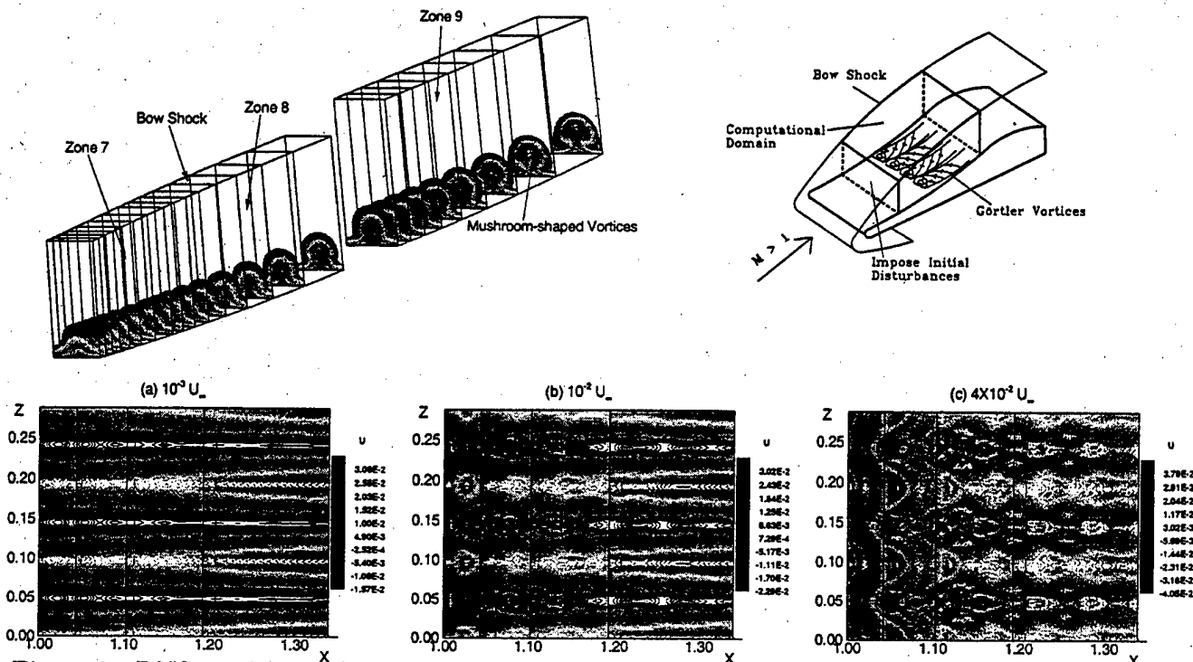
Figure 7: DNS studies of Görtler/second-mode interaction: cross sectional streamwise disturbance contours of Görtler and 2-D second modes at M_\infty = 15 , Re_\infty = 1.5 \times 10^5/m .
