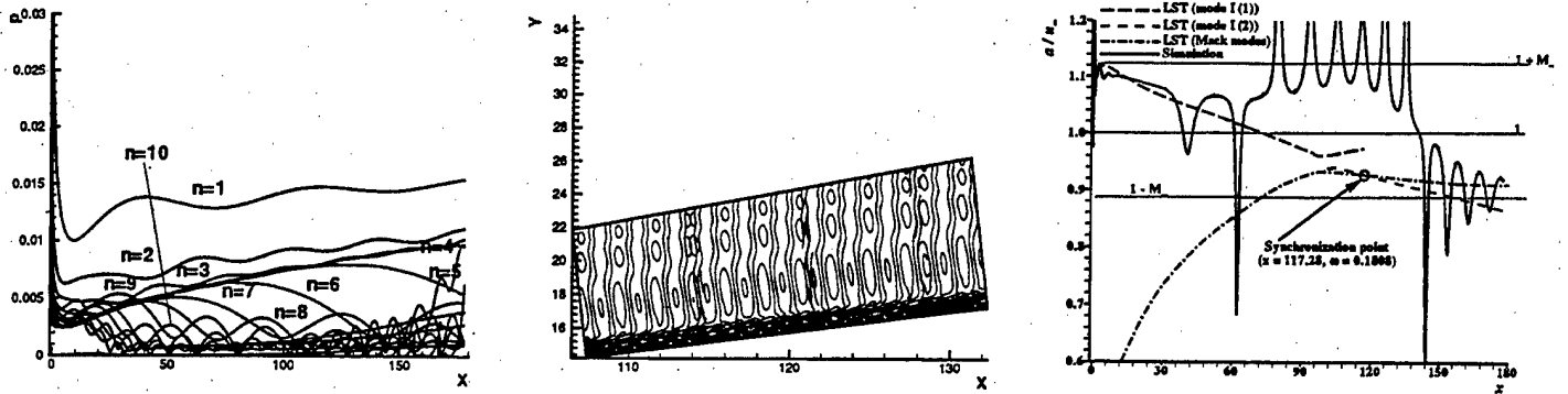
Figure 3: Results of receptivity simulation: 1) pressure perturbations along the cone surface; 2) contours of temperature perturbations ( f^* = 149.2\text{kHz} , n = 10 ); 3) phase velocities along the cone surface at frequencies of n = 10 .
