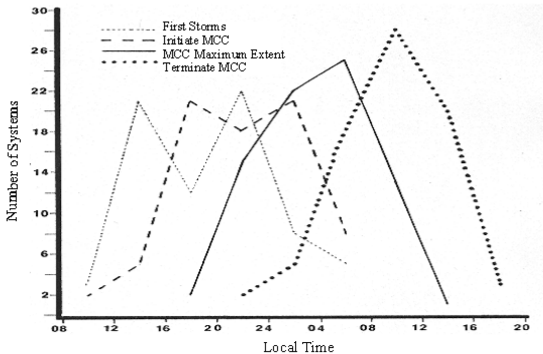
Fig. 18. Average life cycle of mid-latitude South American MCCs from the 1981-82 and 1982-83 austral summers (modified from Velasco and Fritsch 1987).
