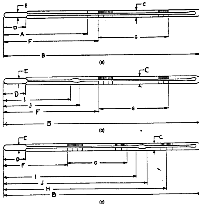
FIG. 1 Thermometer Designs
