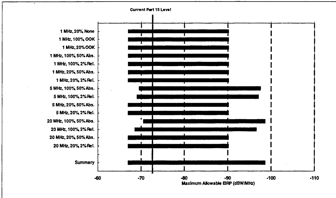
Figure 4-4. Range of Maximum Allowable EIRP for Noise-Like UWB Signal Structures for the C/A-code Receiver Architecture (Multiple UWB Device Operational Scenarios)
