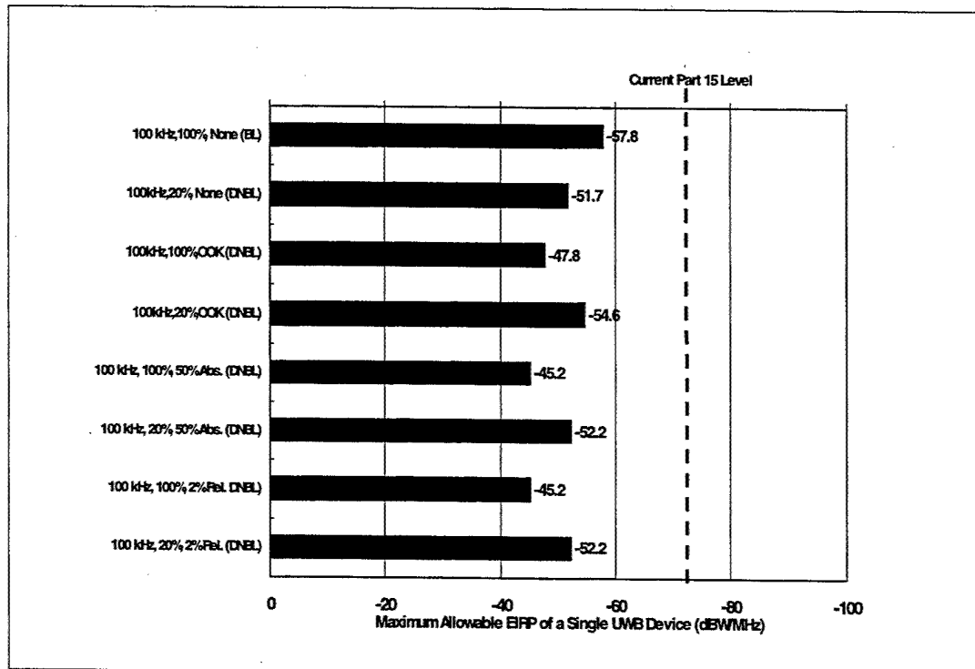
Figure 3-27. Analysis Results for Railway Operational Scenario: C/A-code Receiver and Multiple UWB Devices - Outdoor Operation (Pulse-Like UWB Signals)
