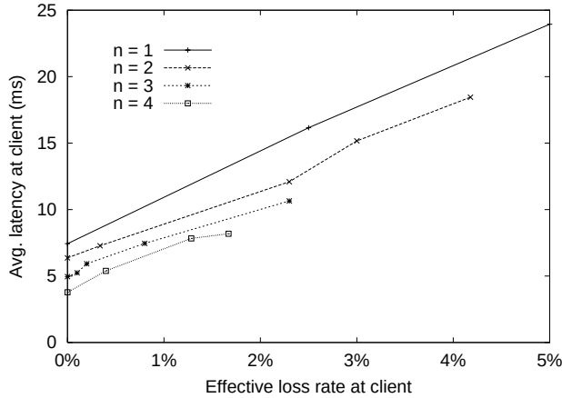
Figure 8: Average per-packet latency from root to client for a range of effective loss rates. Effective loss rates for each level of redundancy are taken from Figure 6.
