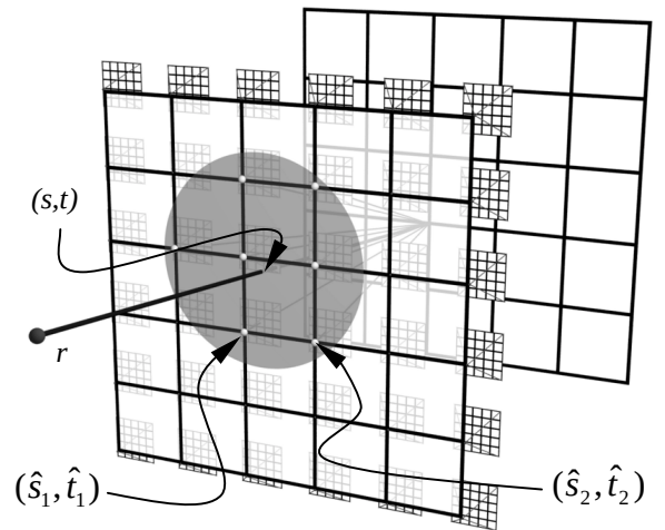
Figure 4: By including rays from all cameras within a radius of the actual camera surface intersection, we can increase the aperture of our synthetic camera.
