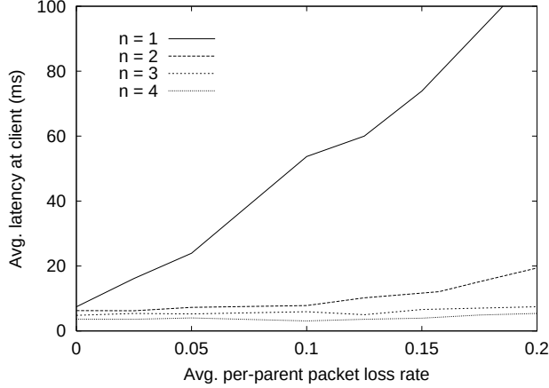
Figure 7: Average per-packet latency from root to client as a function of individual parent loss rates and the number of parents.
