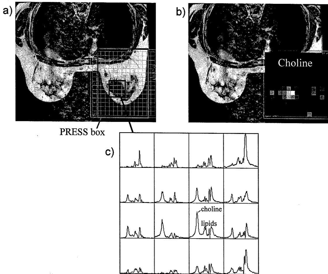
Figure 2. 1 H spectroscopic imaging of breast cancer, same patient as in Figure 1. (a) T1-weighted imaging showing PRESS box and corresponding 16x16 array of 1cc voxels. (b) metabolic map of the choline peak overlaid on the T1-weighted image. (c) spectra from subset of voxels highlighted in (a). High choline is visible within the lesion.
