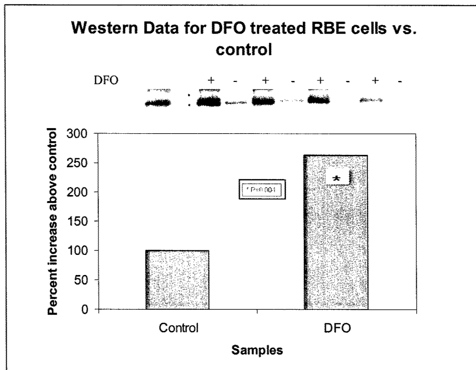
Figure 7. Western blot analysis of DMT-1 in RBE4 cells treated in the presence and absence of desferrioxamine (DFO; 100 uM for 24 hours). Graph depicts the image quantification of the western blots, establishing a statistically
