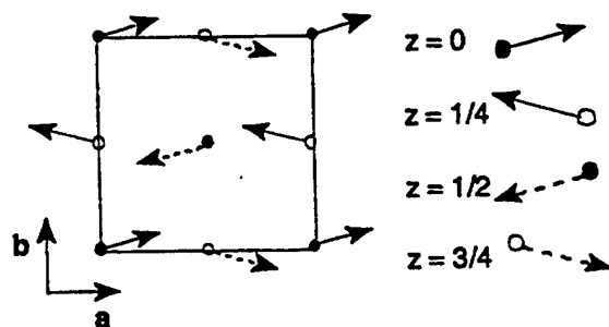
Figure 1 Dipole moments within the AFE unit cell.
