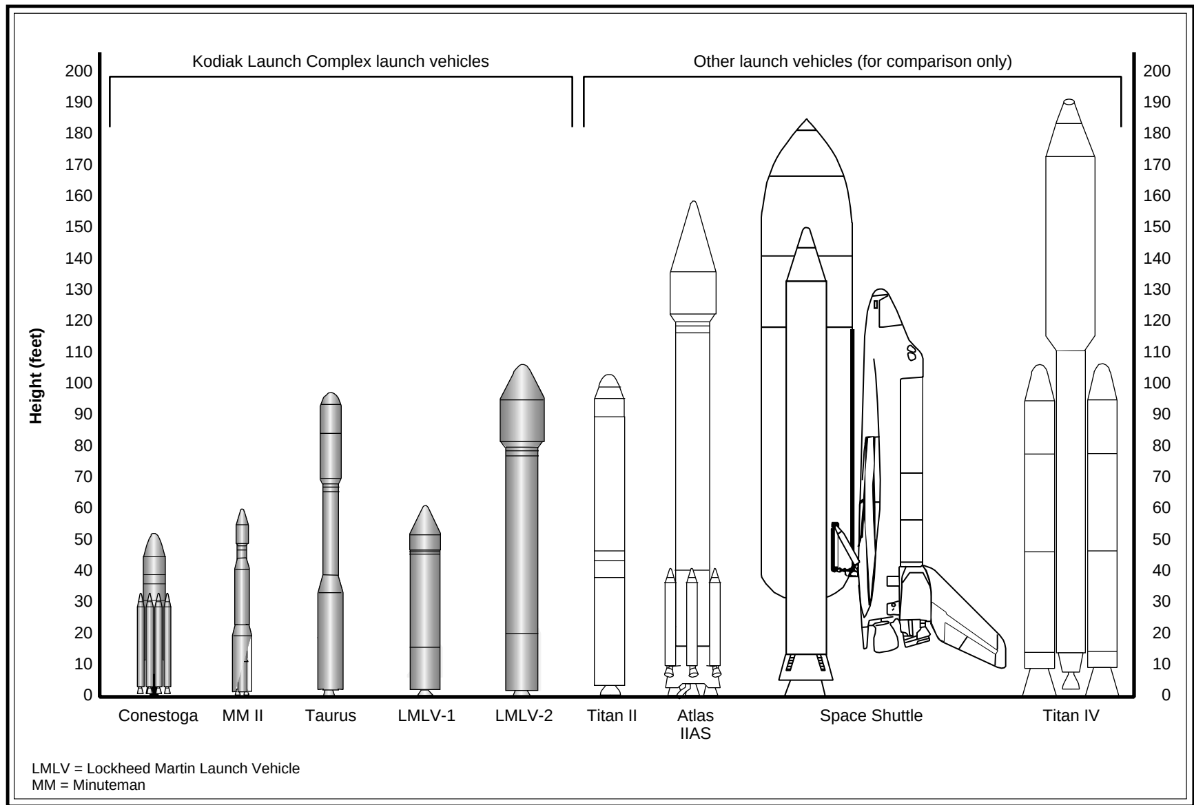
Figure 2.1-14. Representative launch vehicles.
