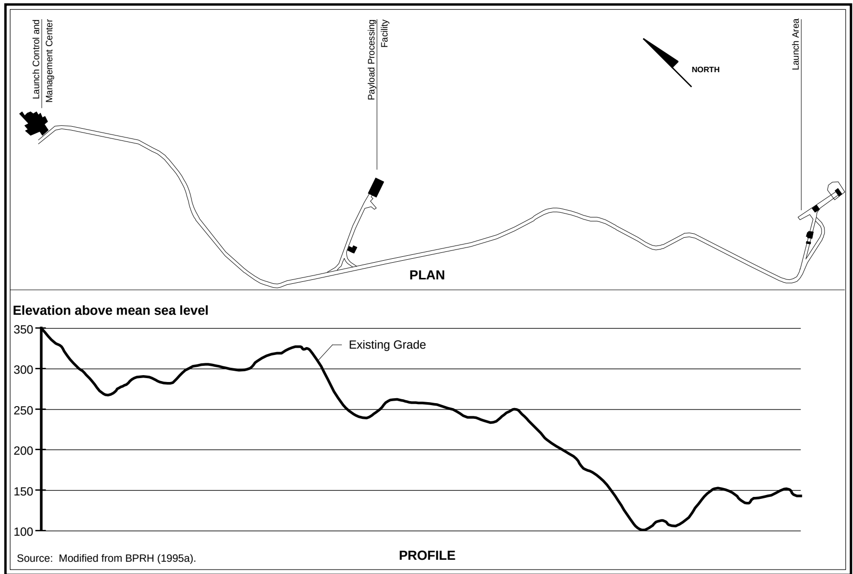
Figure 2.1-8. Pasagshak Point Road plan and profile.
