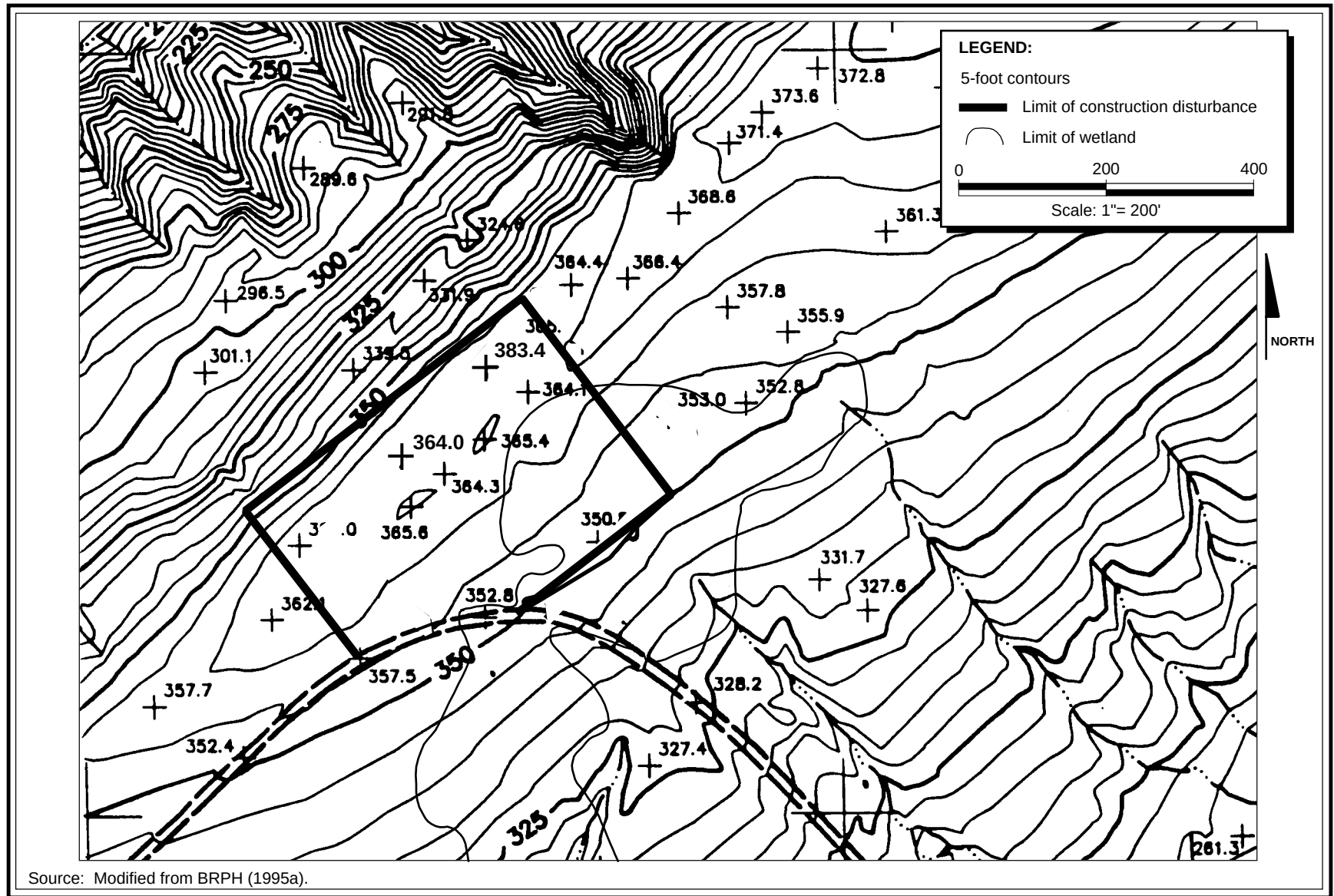
Figure 2.1-4. Proposed Launch Control and Management Center site location.
