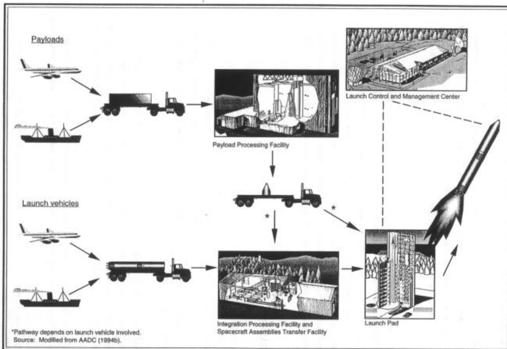
Figure 2.1-10. Proposed KLC operations.
