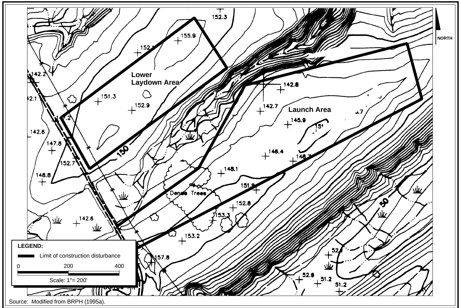
Figure 2.1-6. Proposed Launch Area site location.
