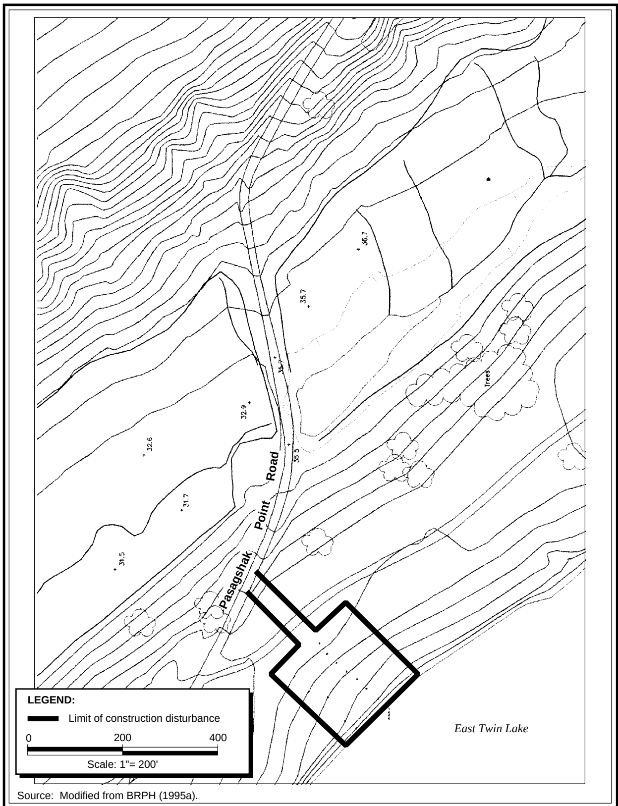
Figure 2.1-7. Proposed Water Pump house site location.
