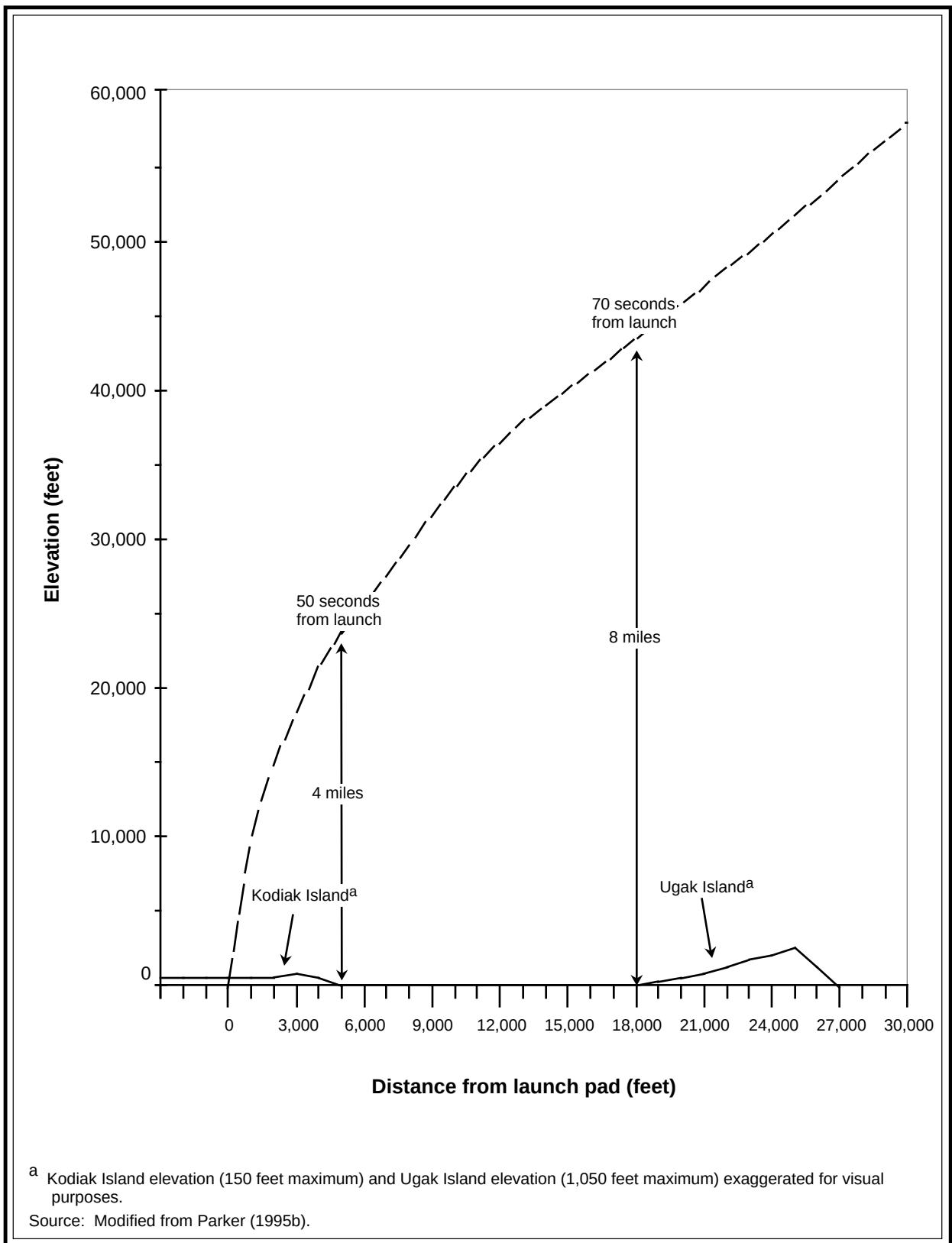
Figure 2.1-16. Launch profile based on Lockheed Martin Launch Vehicle 2.
