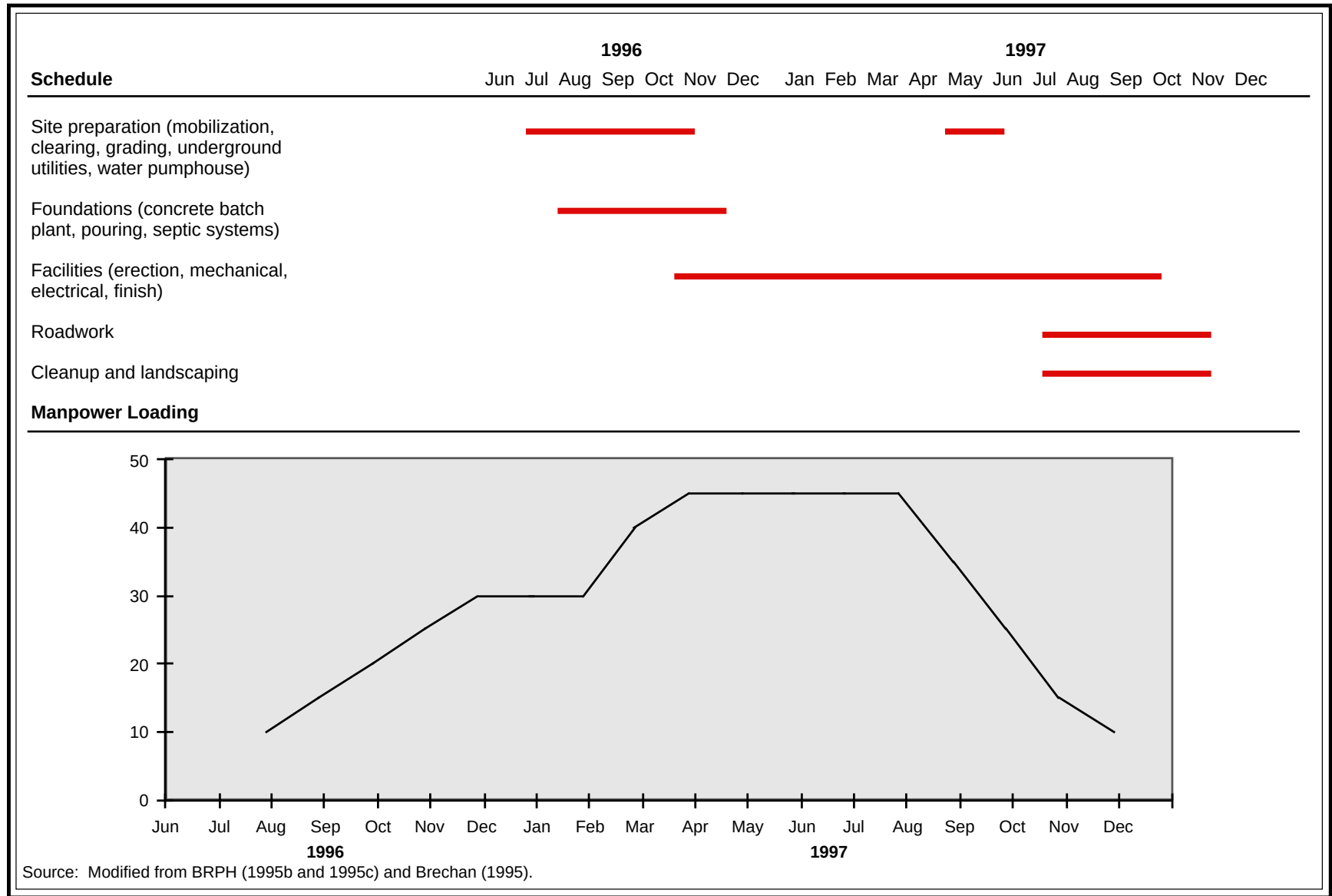
Figure 2.1-3. Construction schedule and manpower loading.
