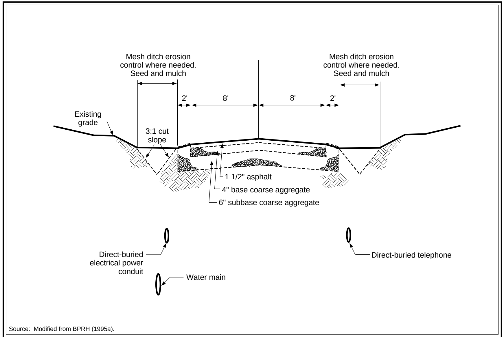
Figure 2.1-9. Pasagshak Point Road typical cross section.
