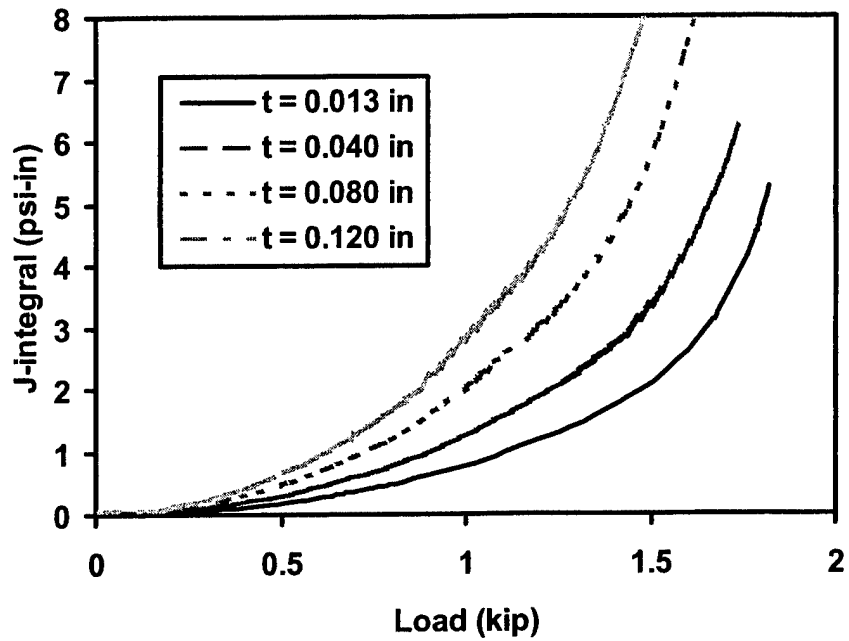
FIGURE 3-55. J-INTEGRAL FOR ASTM D 3165 CONFIGURATION WITH TRIPLE ADHEREND THICKNESS
