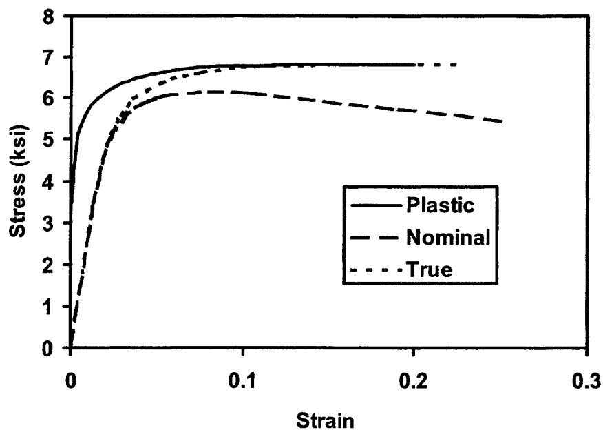
FIGURE 3-2. MATERIAL PROPERTIES OF PTM&W ES6292 PASTE ADHESIVE
