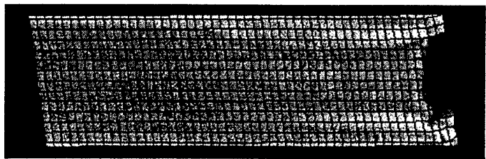
(3) Apparent Shear Strain 0.3136
