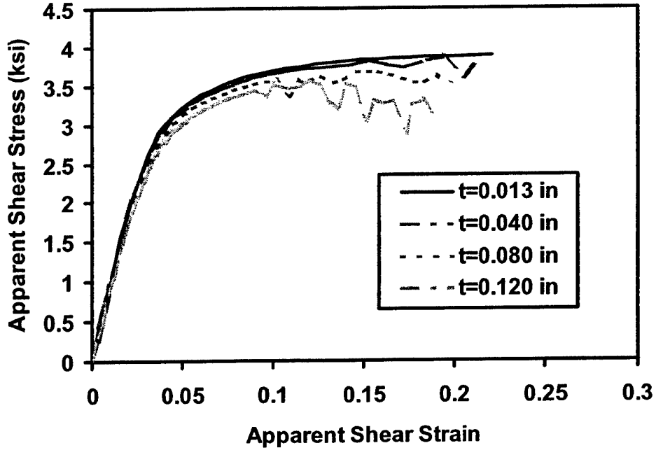
FIGURE 3-28. CALCULATED APPARENT SHEAR STRESS-STRAIN CURVES FOR ASTM D 5656 SPECIMENS
