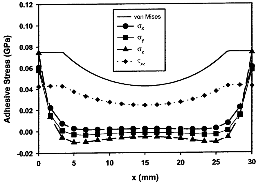
FIGURE 2-3. ADHESIVE STRESS DISTRIBUTION FROM FEM (ABAQUS)
