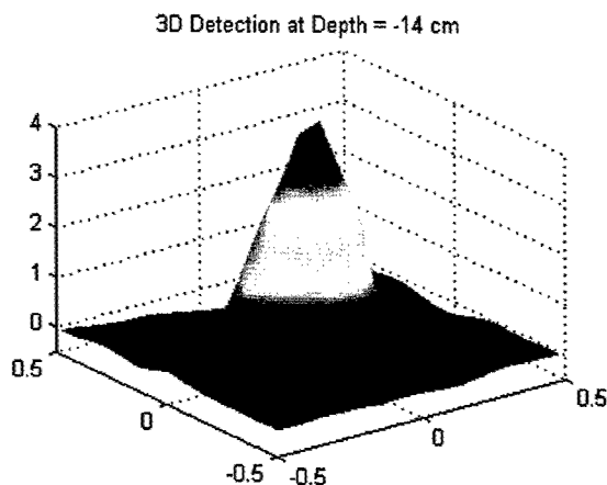
Figure I.2—Detector Response for an Antitank Mine-Like Object Buried at a Depth of 14 cm
