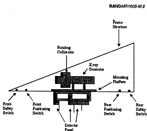
Figure M.2—Drawing of Field Test LMR Mine Detection System (XMIS)
