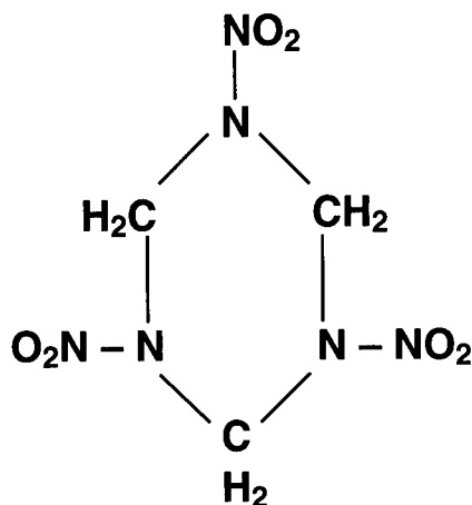
Figure K.3—Chemical Structure of RDX
