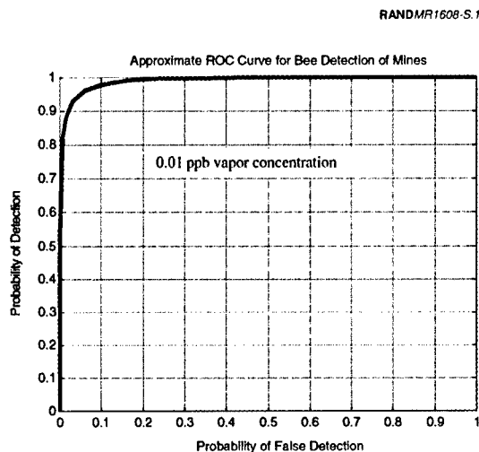
Figure S.1—ROC Curve for Honeybees Trained to Associate the Smell of DNT with Food
