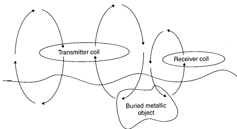
Figure B.1—Typical Electromagnetic Induction System
