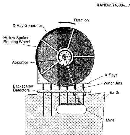
Figure L.3—Illustration of the Standard AS&E Backscatter System Adapted to Work in Conjunction with a Water-Jet Hole Drilling System
