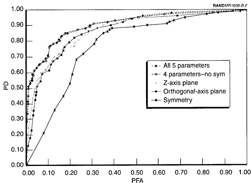
Figure B.2—ROC Curve Results for Modified AN/PSS-12 Sensor
