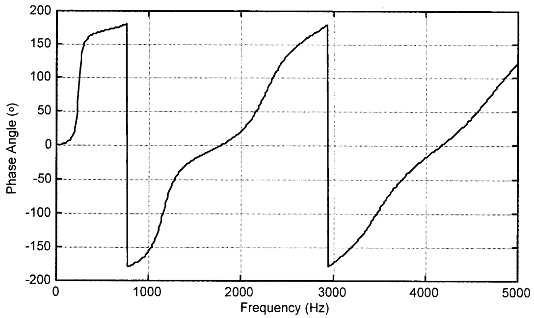
Figure 14. Transfer Function of Horizontal Motion Versus Frequency for System with Mass
