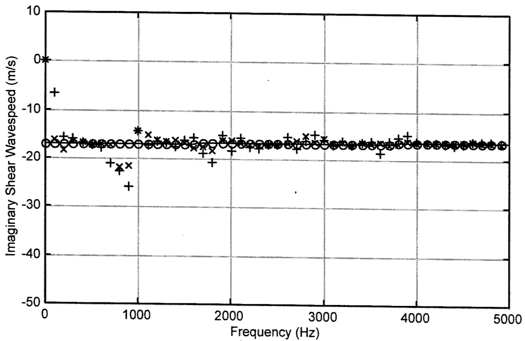
Figure 9. Actual and Estimated Shear Wavespeed Versus Frequency for System Without Mass
