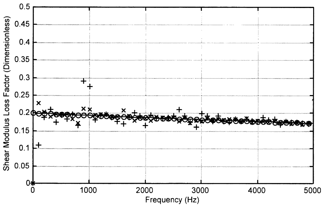
Figure 10. Actual and Estimated Shear Modulus Versus Frequency for System Without Mass
