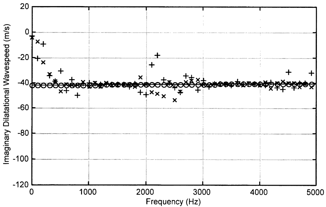
Figure 8. Actual and Estimated Dilatational Wavespeed Versus Frequency for System Without Mass
