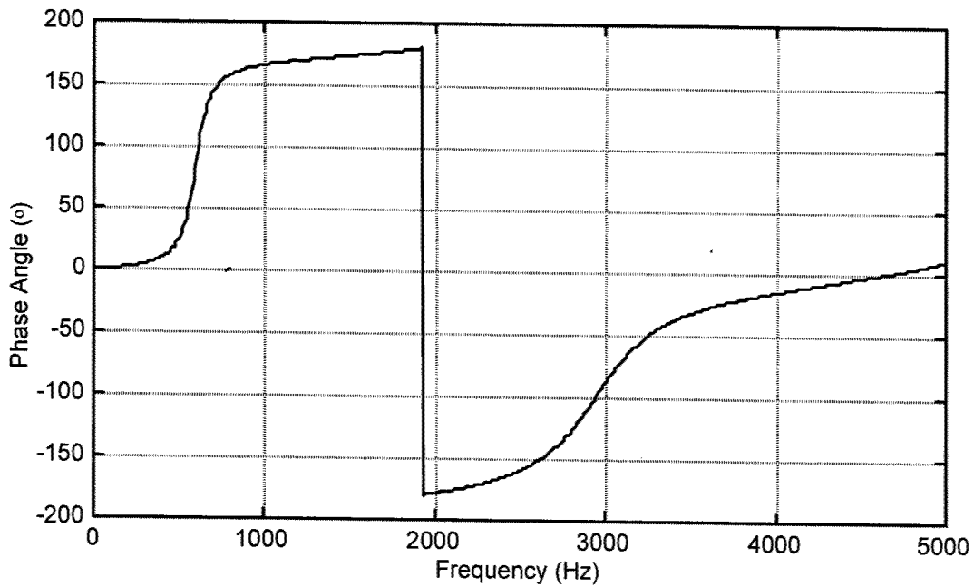
Figure 13. Transfer Function of Vertical Motion Versus Frequency for System With Mass
