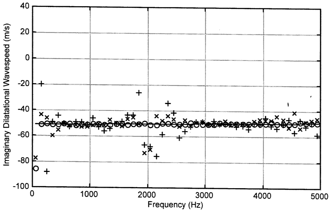
Figure 17. Actual and Estimated Dilational Wavespeed Versus Frequency for System with Mass
