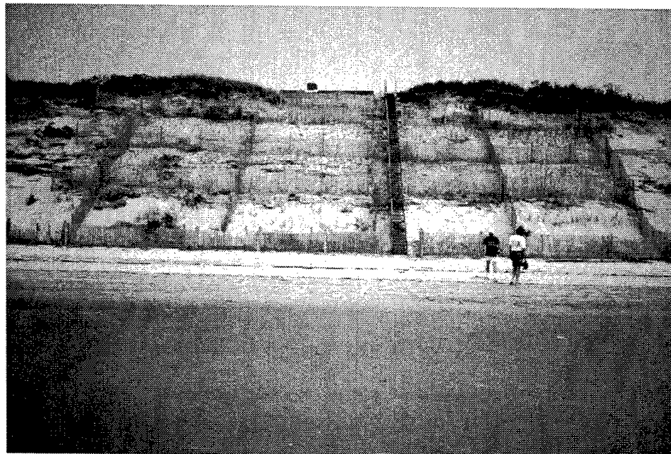
Fig 2. Partially successful non-structural erosion control on a coastal bank
