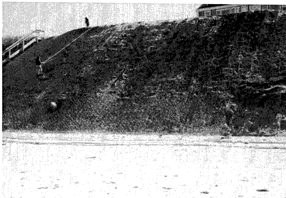
Fig 28. Coastal bank with fill and jute netting being planted
