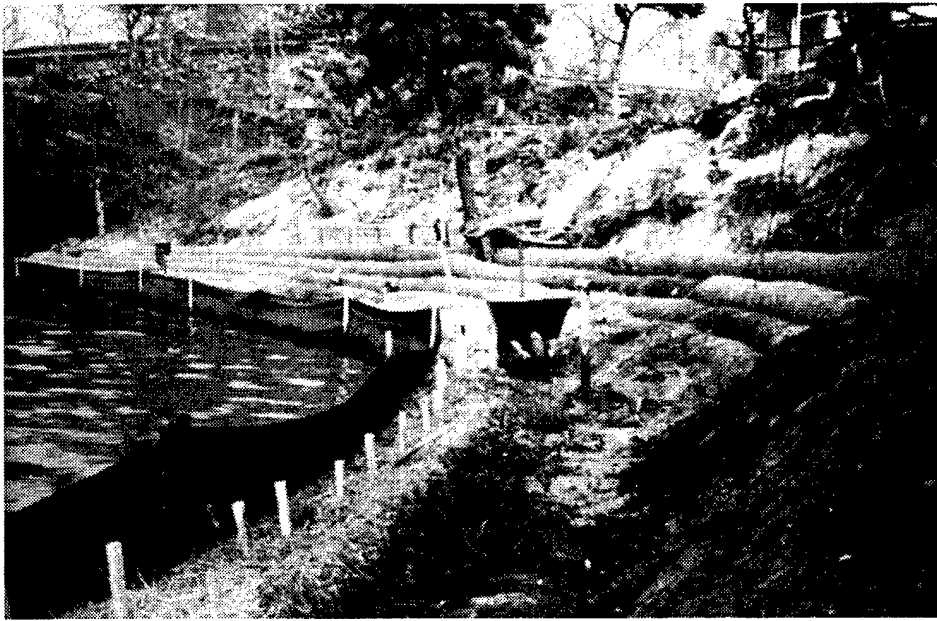
Fig 33. Bournes Pond bank stabilization under construction
