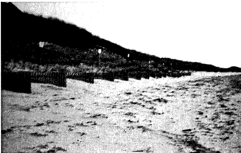
Fig 24. Coastal bank stabilization with plants and a drift fence
