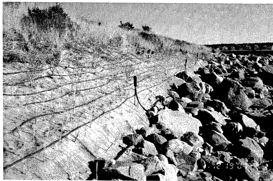
Fig 7. Coastal bank erosion control using bioengineering (bio-logs, jute netting, plants) and a system for watering and fertilizing
