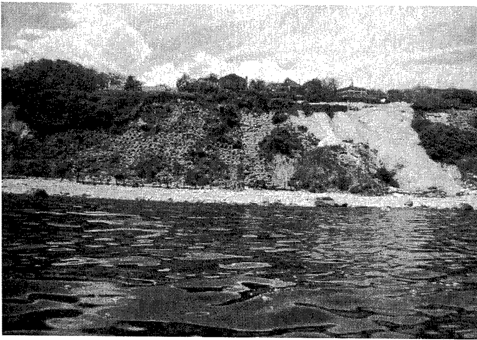
Fig 1. Innovative non-structural erosion control methodology on a coastal bank: A matrix of hay bales
