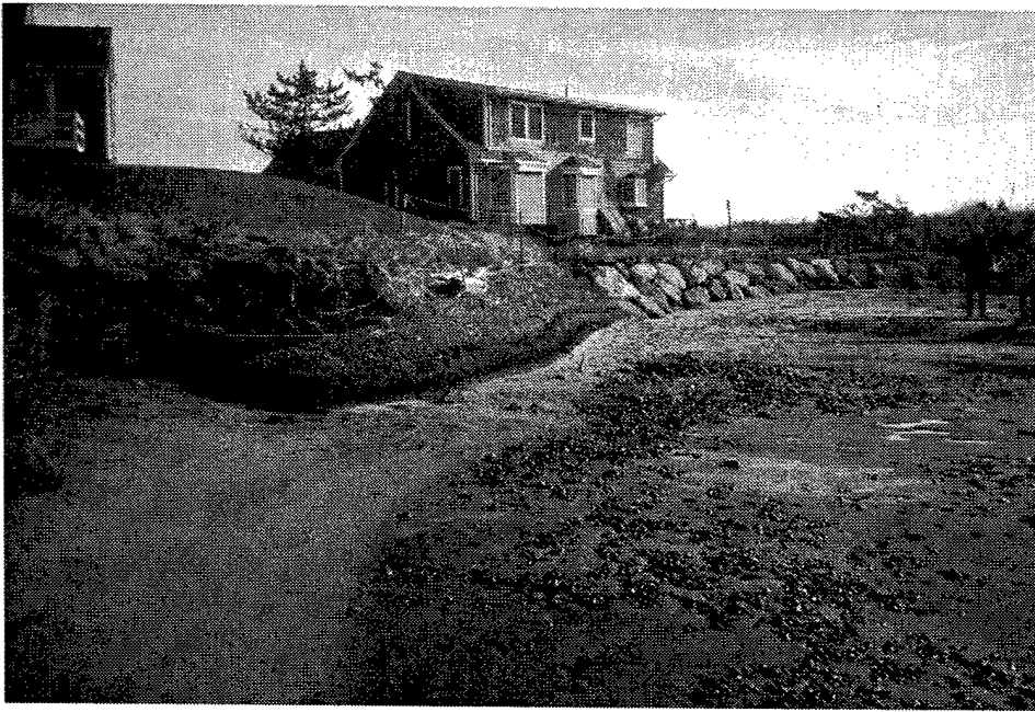
Fig 6. End scour on flanking erosion around bio-logs
