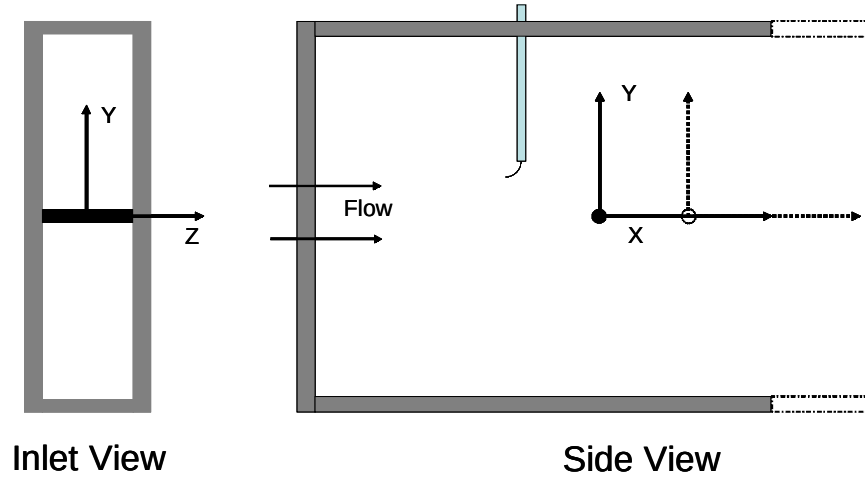
Figure 2.2 Single Cylinder Test Section
