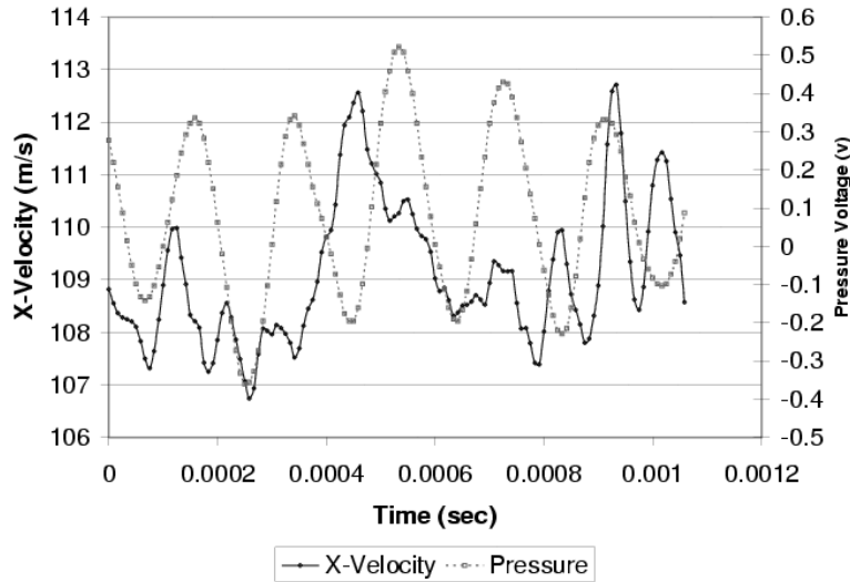
Figure 2.6 Single Trace with Probe 1/2 inch Upstream and 1/4 inch Above Centerline
