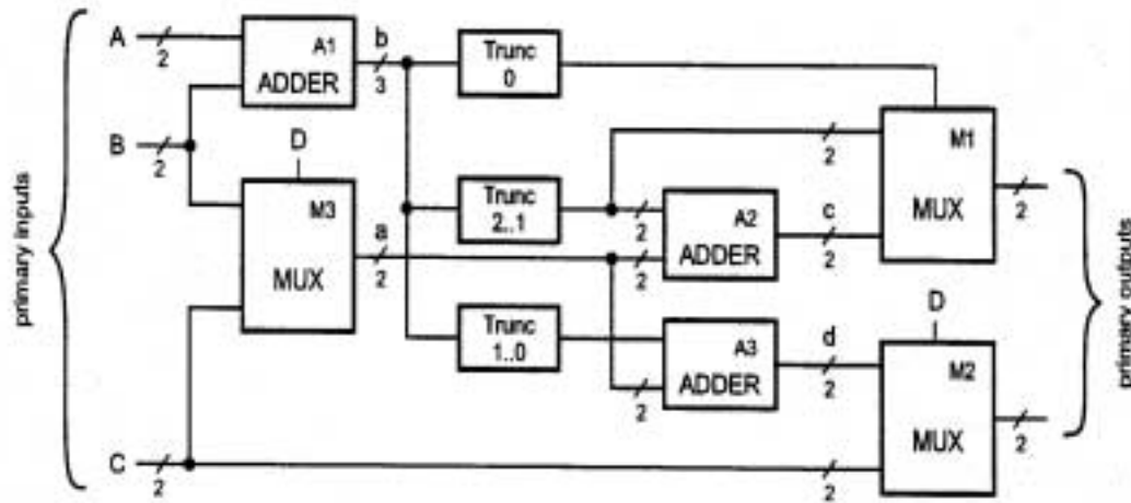
Figure 2-12. Electrical schematic [14]
