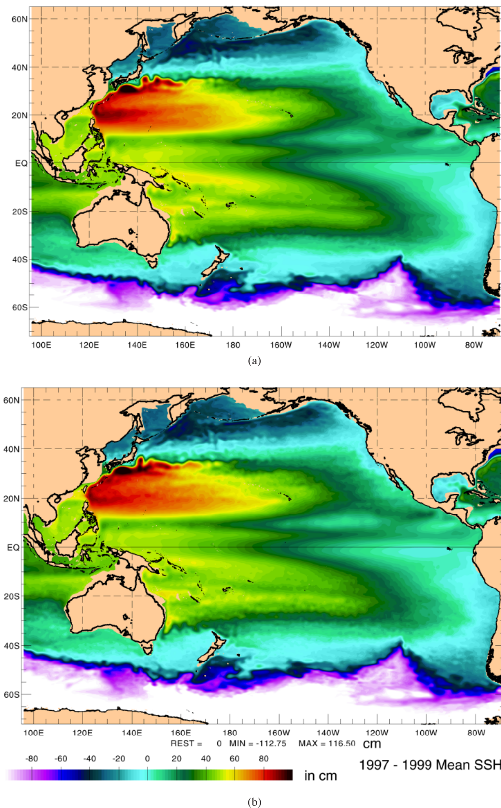
Fig. 1 — The 1997-1999 mean Pacific hemispheric SSH for (a) the non-assimilative 1/16° global NLOM and (b) the data-assimilative 1/16° global NLOMI. NLOM is forced with NOGAPS wind and thermal fields.
