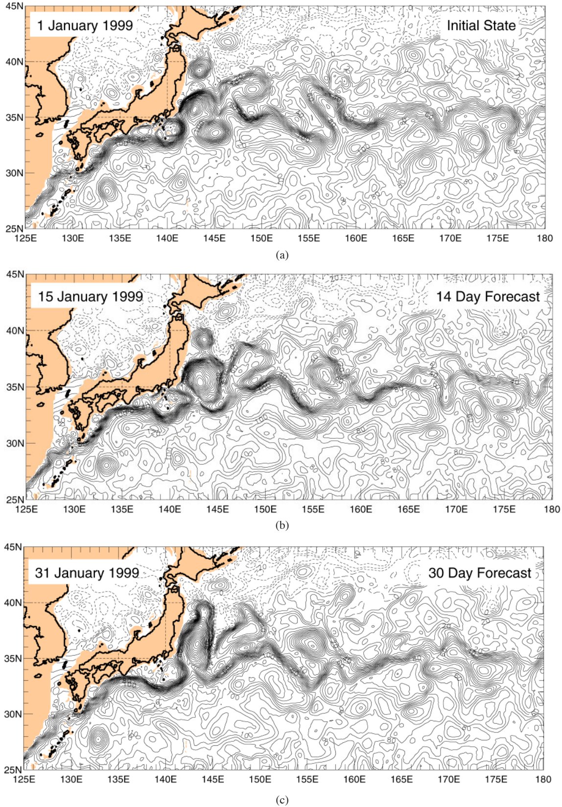
Fig. 32 — SSH for the Kuroshio region from the 1/16° global NLOM running in forecast mode for a 30-day forecast. The model forecast was initialized on 1 January 1999 (a) and forecasts are shown for (b) 15 January 1999 and (c) 31 January 1999. The model was forced with FNMOC wind and thermal fields gradually interpolating to climatological forcing for the long-term forecast.
