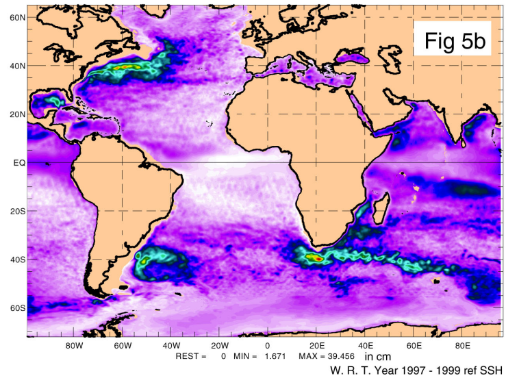
Fig. 5 — The 1997-1999 SSH variability in the Atlantic/Indian hemisphere for (a) the non-assimilative 1/16^\circ global NLOM, (b) the assimilative 1/16^\circ global NLOM, and (c) TOPEX/Poseidon altimetry. NLOM is forced with NOGAPS wind and thermal fields.
