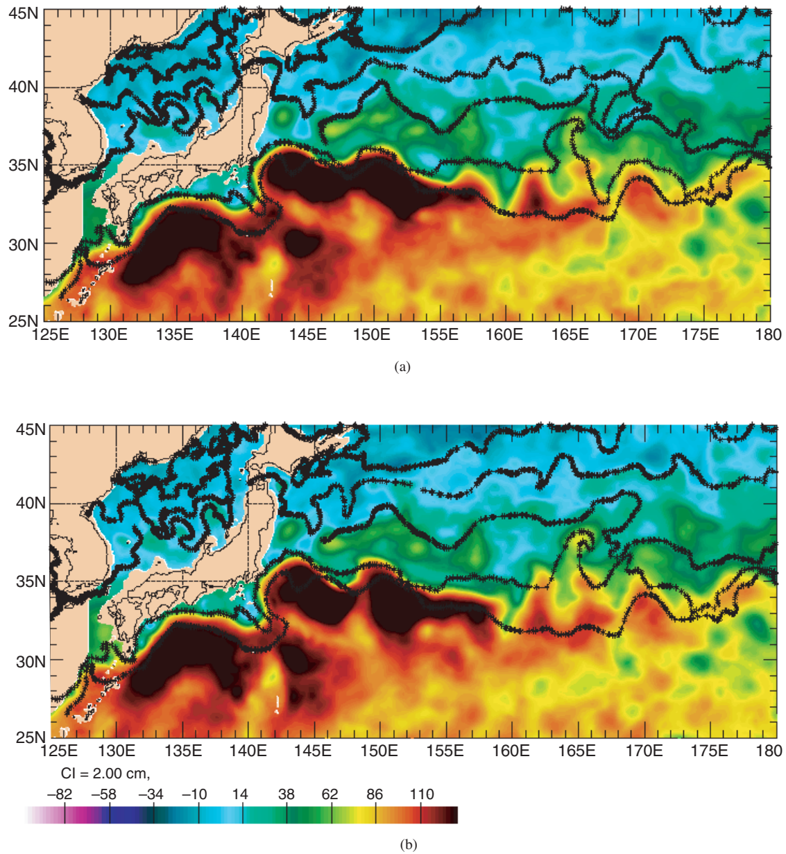
Fig. 14 — SSH analysis (nowcast) in the Kuroshio region from the assimilative 1/16^\circ global NLOM for (a) 20 October 2000 and (b) 30 October 2000. Superimposed on each is the frontal analysis determined from satellite IR imagery (black lines) from the Naval Oceanographic Office for the same day.
