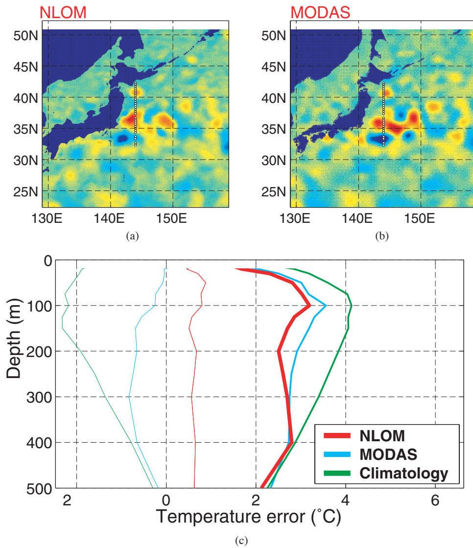
Fig. 20 — SSH anomalies with respect to a long term mean for (a) assimilative 1/16^\circ global NLOM and (b) 1/8^\circ global MODAS OI analysis from the Naval Oceanographic Office for 20 July 1999. Superimposed on with mean (thin lines) and RMS (thick lines) temperature error statistics for synthetic profiles as function of depth from NLOM-derived synthetics (red lines), MODAS-derived synthetics (blue lines), and MODAS climatological temperature (green lines).
