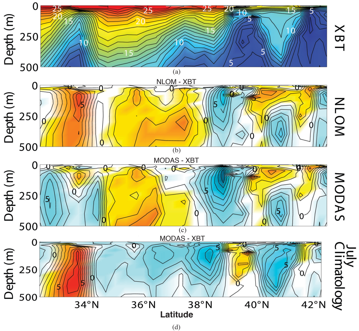
Fig. 22 — Observed XBT data (a) along a section at 144° E on 16-22 July 1999 from the surface to 500-m depth and temperature error cross-sections for (b) MODAS synthetic profiles derived from 1/16° global NL0M SSH field-XBT data, (c) MODAS synthetic profiles derived from 1/8° global MODAS SSH field-XBT data, and (d) July climatological temperature from MODAS-XBT data.
