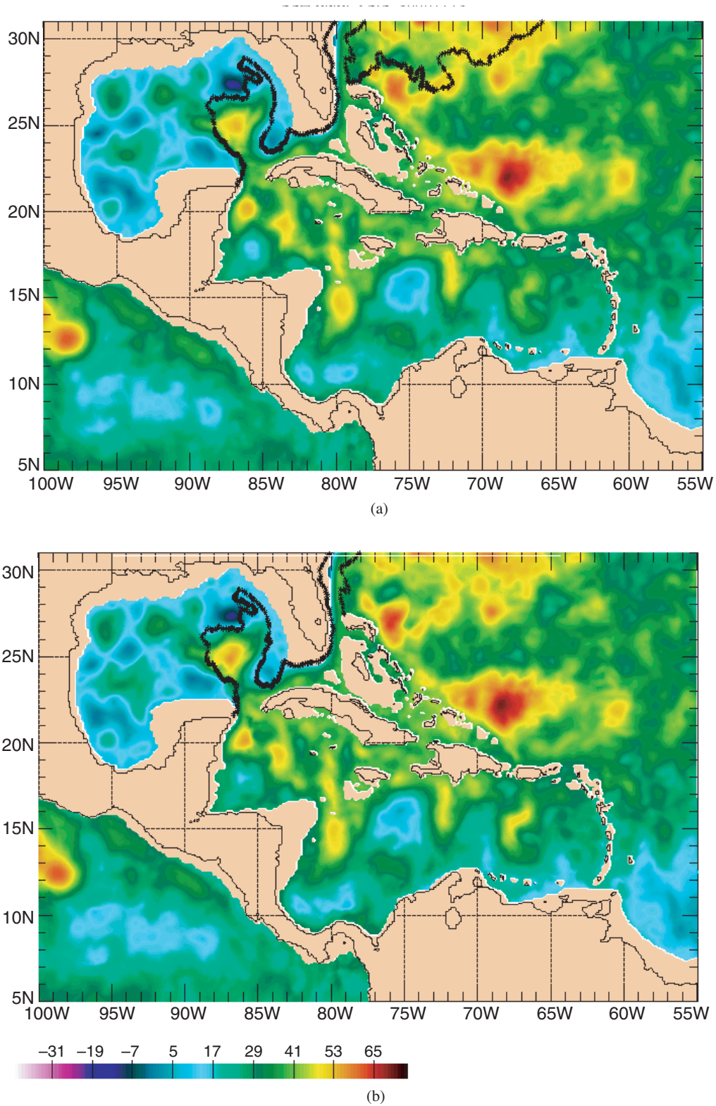
Fig. 18 — SSH analysis (nowcast) in the Intra-Americas Seas region from the assimilative 1/16° global NLOM for (a) 13 November 2000 and (b) 15 November 2000. Superimposed on each is the frontal analysis determined from satellite IR imagery (black lines) from the Naval Oceanographic Office for the same day.
