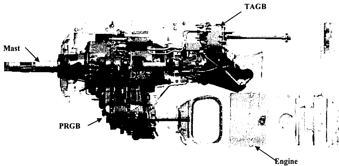
Figure 3.—Layout view of typical tiltrotor nacelle (airplane mode).
