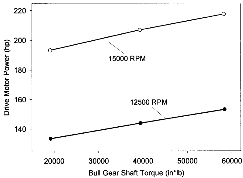
Figure 8.—Drive motor power required at high speed and load.
