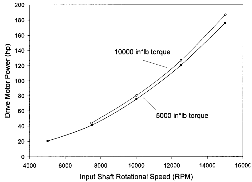
Figure 7.—Drive motor power required to rotate the entire test facility as a function of input shaft speed (bull gear shaft torque shown).
