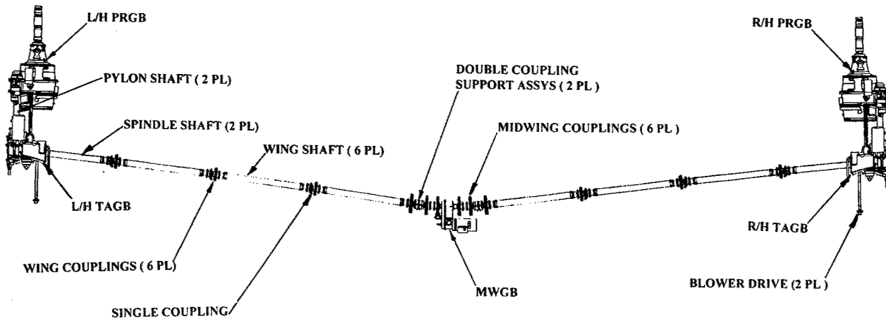
Figure 2.—Typical tiltrotor drive system arrangement.
