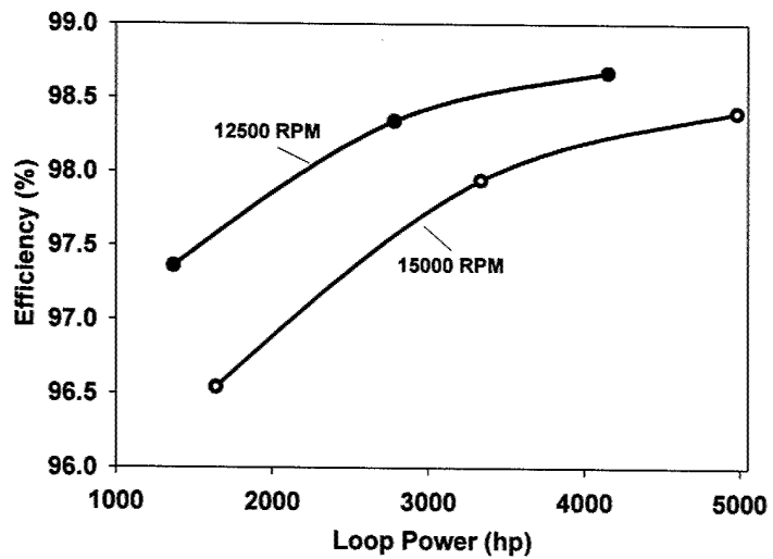
Figure 14.—Analytical prediction of high speed helical gear train efficiency at high speed and load.
