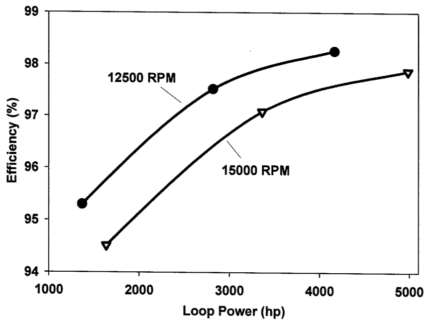
Figure 10.—Effect of high speed and load on helical gear train performance.
