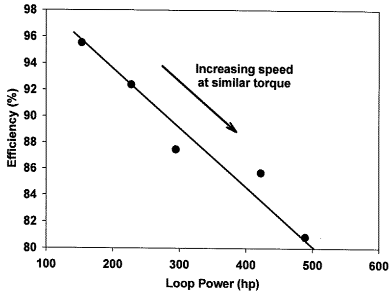
Figure 9.—Effect of shaft speed (input shaft speed: 5,000 to 15,000 rpm) at similar light load.
