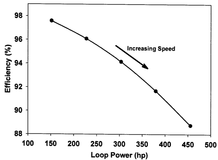
Figure 13.—Analytical prediction of the high speed helical gear train efficiency.
