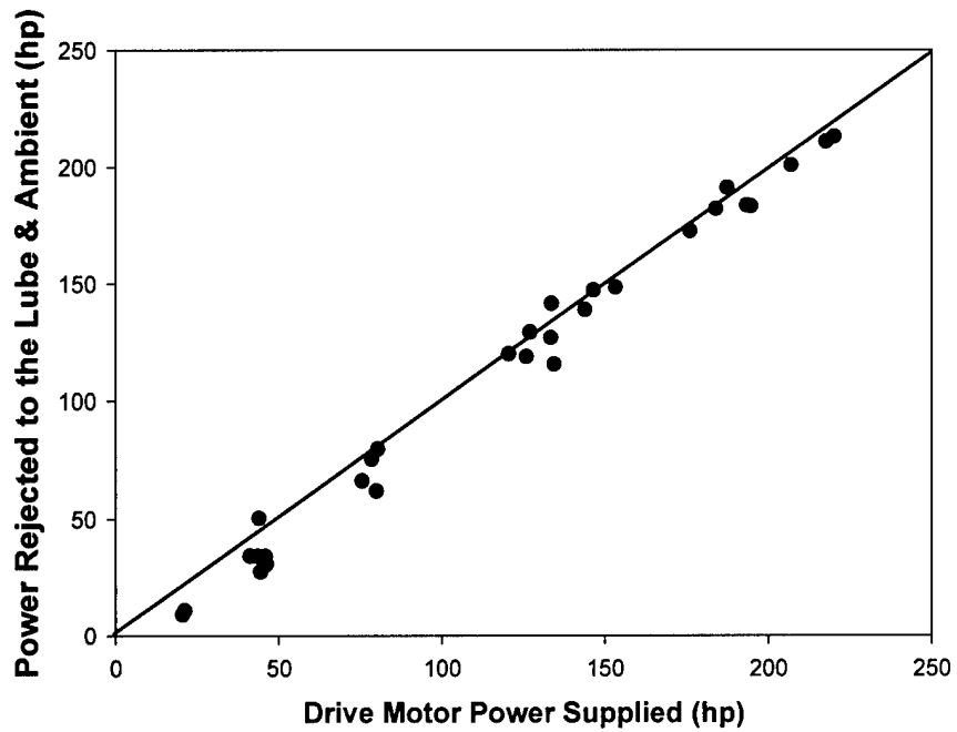
Figure 11.—Comparison of supplied power versus calculated power rejected for both the test and slave gearboxes.
