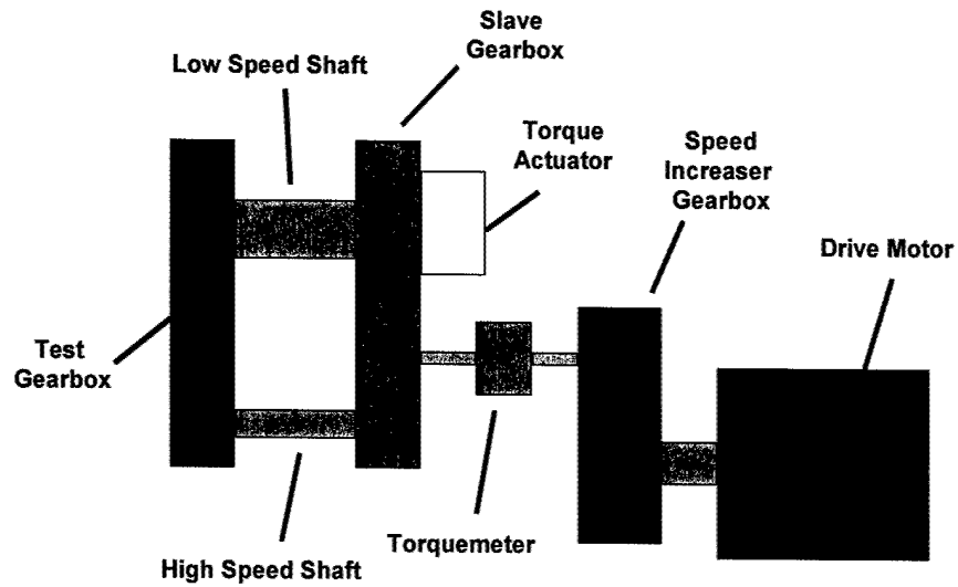
Figure 5.—Layout of NASA High-Speed Helical Gear Train Test Facility.
