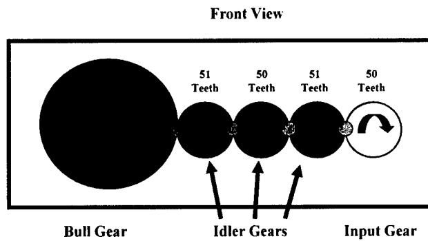
Figure 12.—Layout of helical gear train arrangement.
