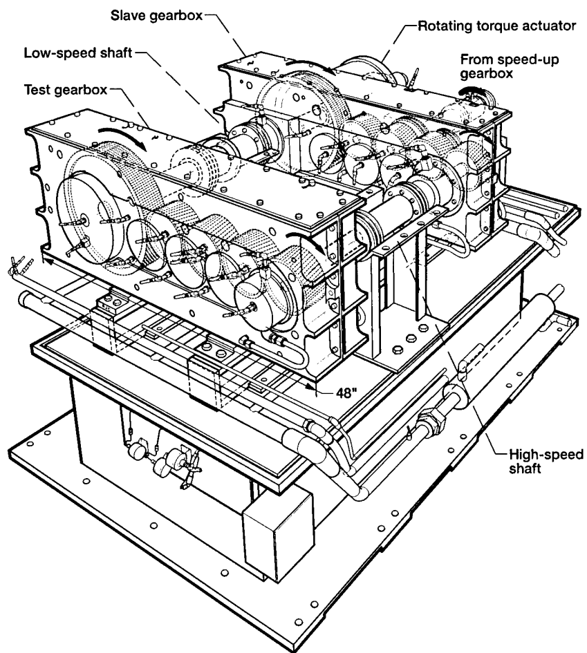
Figure 4.—NASA High-Speed Helical Gear Train Test Facility.
