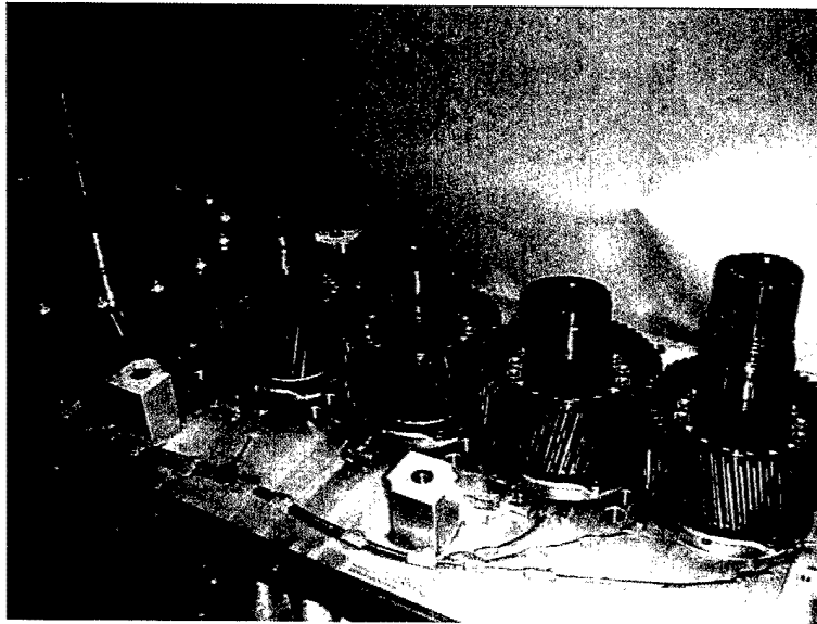
Figure 6.—NASA High-Speed Helical Gear Train Test Facility Components.
