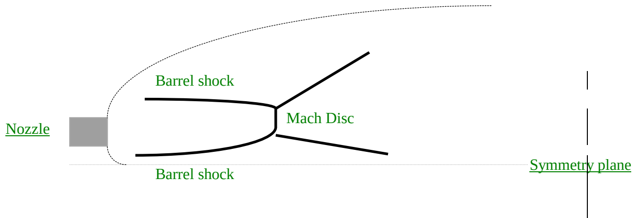
Figure 2.2a – Flow Structure of a Twin Supersonic Plume: Top View
