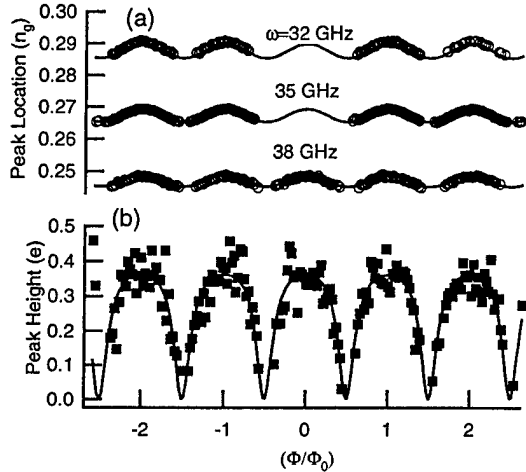
FIG. 3: (a) The locations of resonant peaks (circles) in n_g and \Phi , for \omega = 32, 35, and 38 GHz and fits (lines), using Eq. 1 for \omega_{01} = 2\omega = 64, 70 and 76 GHz to find single value of E_C and of E_J^{max} . The systematic uncertainty in n_g is represented by the size of the open circle symbols. (b) The height, in electrons, of a 76 GHz resonant peak as a function of \Phi (squares) and a guide to the eye (line).
