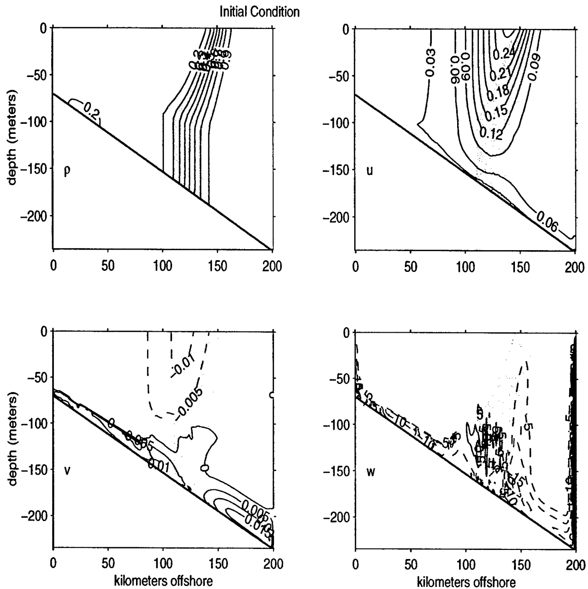
Figure 2-19: The initial condition experiment, a slice through the channel at x=200 km, after 230 days. In this experiment, there density driven jet is superimposed on a barotropic inflow of 2.5 \text{ cm/s} and there is no wind stress. (a) density anomaly ( \text{kg m}^{-3} ) (b) along-channel velocity, positive downstream ( \text{m/s} ) (c) cross-channel velocity, positive offshore ( \text{m/s} ) (d) vertical velocity, positive up ( \text{times } 10^6 \text{ m/s} ). To reduce the contours, the 0 contour was eliminated from the w plot. In all figures, the location of the front is shaded. Dotted contours indicated negative values. Note the well developed bottom mixed layer.
