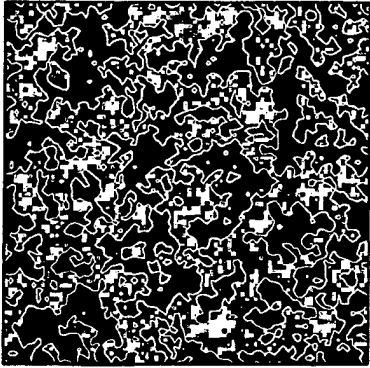
Figure 13. Snapshot of forest-fire simulation.
