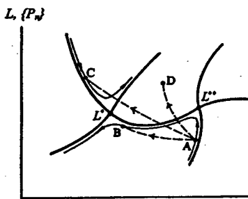
Figure 11. Renormalization-group trajectories and fixed points.
