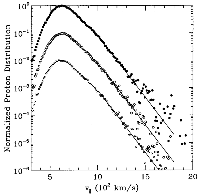
Figure III.2.8: Cuts of normalized proton velocity distributions at the v_{\perp} = 0 plane at 0.2 AU. The crosses ( \times ) corresponds to the solution based on a Maxwellian approximation for the total electron population. Open circles ( \circ ) are for the solution that includes kinetic suprathermal electron effects. The ratio e_{-}/e_{+} is given by Eq. (III.2.5) for both of these cases. Filled circles ( \bullet ) are for e_{-}/e_{+} given by Eq. (III.2.26), with suprathermal electron effects considered. For clarity, the distributions are normalized differently so that their peak values are exactly one order of magnitude apart. The straight solid lines at the tail of the distributions are parallel and also exactly one order of magnitude apart.
