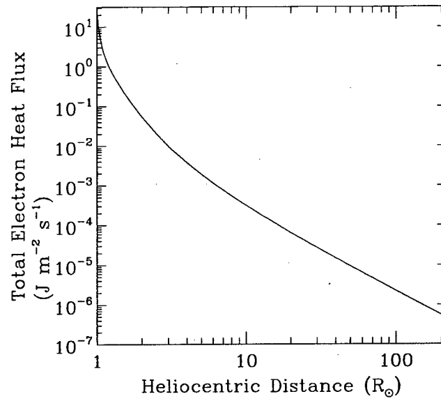
Figure III.2.3: Profile of the total electron heat flux from 1 R_{\odot} to 1 AU in the case where the kinetic effects of the suprathermal electrons are included. The meaning of the thick line segment and the cross ( \times ) is similar to that in Fig. III.2.2.
