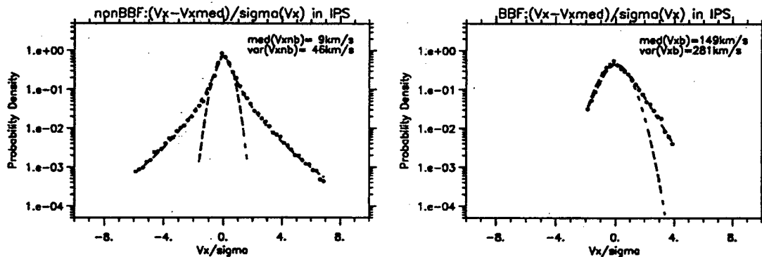
Figure 9. Probability distributions of the non-BBF and BBF x-component of the normalized flows along with best fits of Gaussian and Castaing functions.
