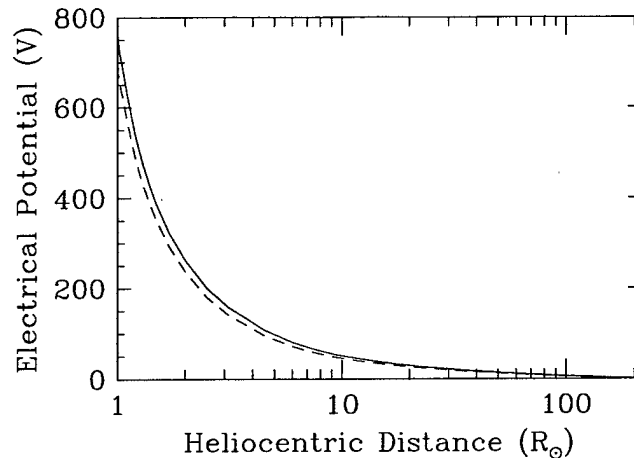
Figure III.2.4: Ambipolar electric potential profiles. Solid line: kinetic suprathermal electron effects included; dashed line: with a Maxwellian approximation for the entire electron distribution.
