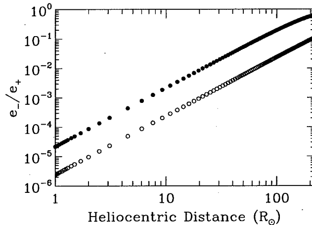
Figure III.2.9: The ratio of sunward to anti-sunward propagating wave power. Open circles: based on Eq. (III.2.5); filled circles: based on Eq. (III.2.26).
