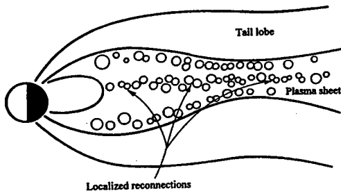
Figure 1. Cross-sectional view of flux tubes in the plasma sheet of the Earth's magnetotail
