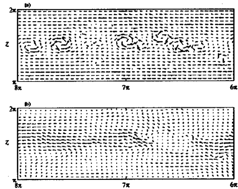
Figure 5. Effect of Lorentz force on coherent structures in a sheared field.
