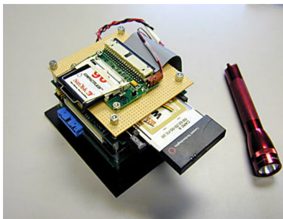
Figure 1. An exposed module is shown next to a 3-inch flashlight.
