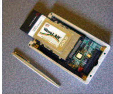
Figure 5: Second generation module processing core.
