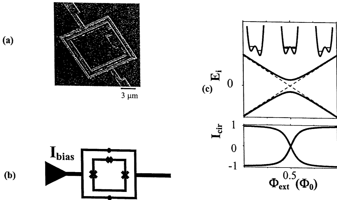
FIGURE 1. (a) SEM image of the persistent current qubit (inner loop) surrounded by the measuring dc SQUID. (b) a schematic of the qubit and measuring SQUID, the x's mark the Josephson junctions. (c) The energy levels for the ground state (dark line) and the first excited state of the qubit versus applied flux. The double well potentials are shown schematically above. The lower graph shows the circulating current in the qubit for both states as a function of applied flux. The units of flux are given in terms of the flux quantum.
