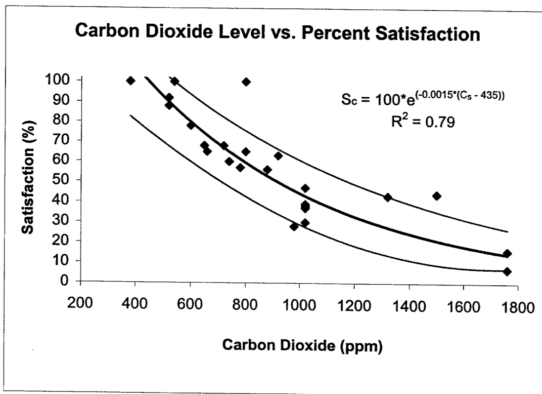
Figure 1. Rate of satisfaction of building environment based on physiological effects of carbon dioxide.
