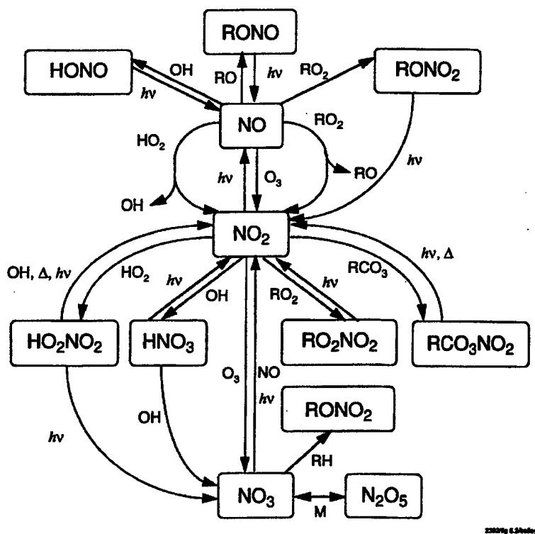
Figure 6 – Tropospheric Chemistry of NO x 23
