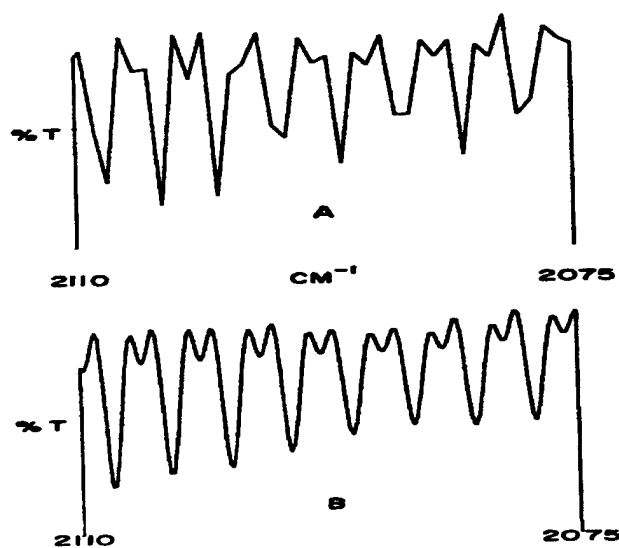
Figure 16 - Effect of Zero-filling on Spectrum of \text{CO}^{122} A. - Raw Spectrum B. - Zero-Filled Spectrum
