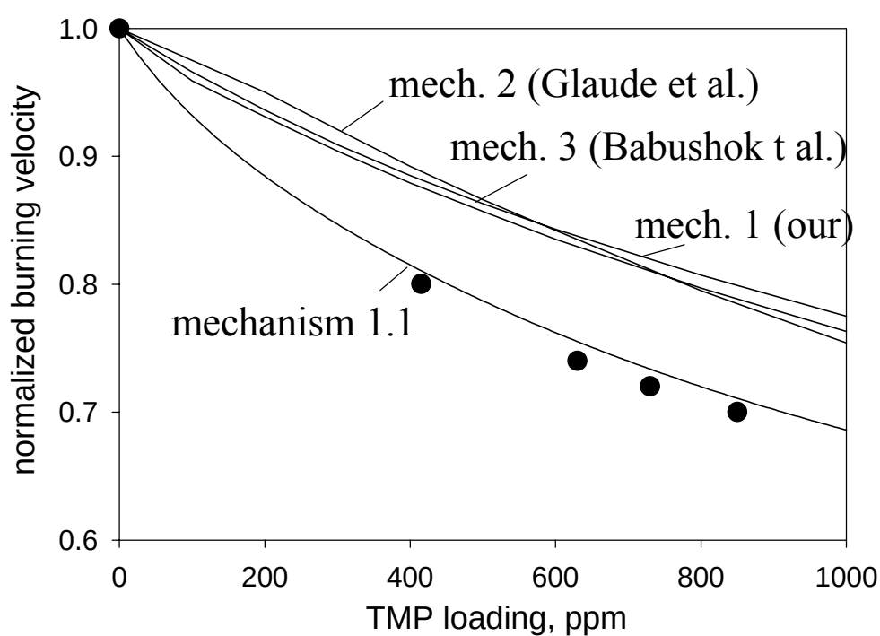
Fig. 25. TMP loading dependence of burning velocity of a stoichiometric CH 4 /air. Symbols - experiment; lines - modeling performed using GRI 3.0 mechanism and mechanisms 1,2, 3 and mechanism 1.1 with modified rate constant \text{H} + \text{PO}_2 + \text{M} = \text{HOPO} + \text{M} , A = 4.0 \times 10^{25} .
