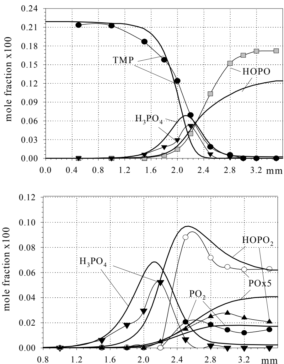
Fig. 13 Concentration profiles of TMP and phosphorus containing products of its destruction in the rich CH_4/O_2/Ar (0.075/0.125/0.80) and sum of experimentally measured concentration of TMP, H_3PO_4 , HOPO_2 , HOPO , PO_2 , PO_{x5} . Solid lines – modeling; symbols – experiment.
