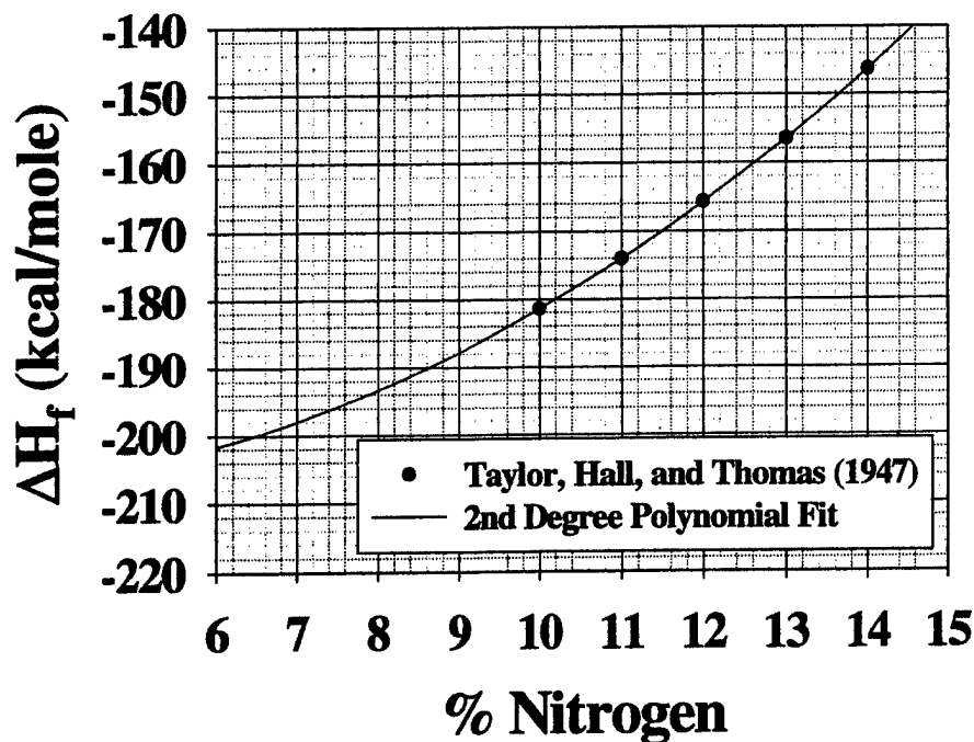
Figure 4. Heats of formation of nitrocellulose as a function of percent nitration generated as an analytic fit to the measurements of Taylor et al. 10
