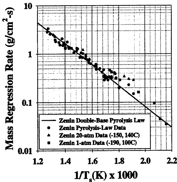
Figure 11. Applicability of Zenin's pyrolysis law 3 to double-base propellants for extreme initial propellant temperatures. 3,32
