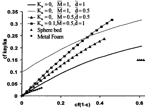
Fig. 12 Orthogonal weave screen laminate conductivity.
