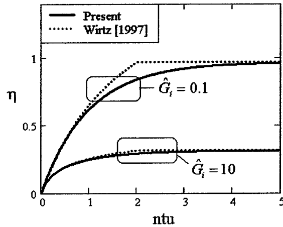
Fig. 3 Comparison of porous models.
