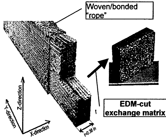
Fig. 34 Three-D woven/bonded mesh fabrication sequence.
