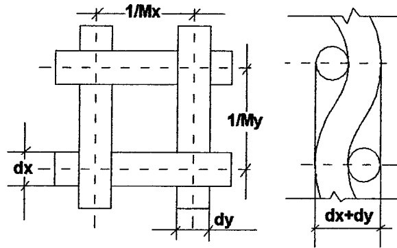
Fig.6 Orthogonal weave unit cell
