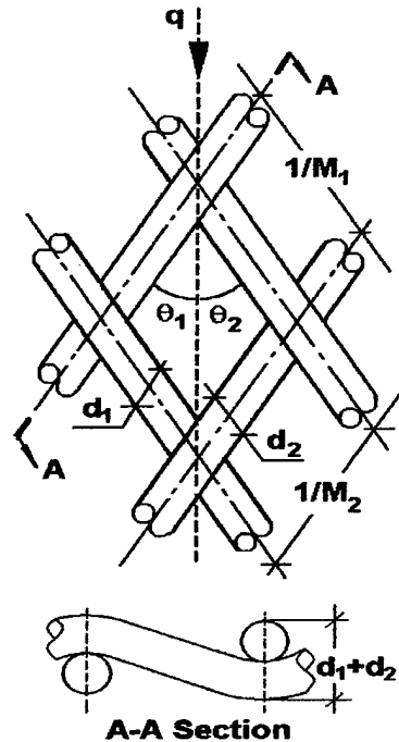
Fig. 20 Diamond-weave unit cell.
