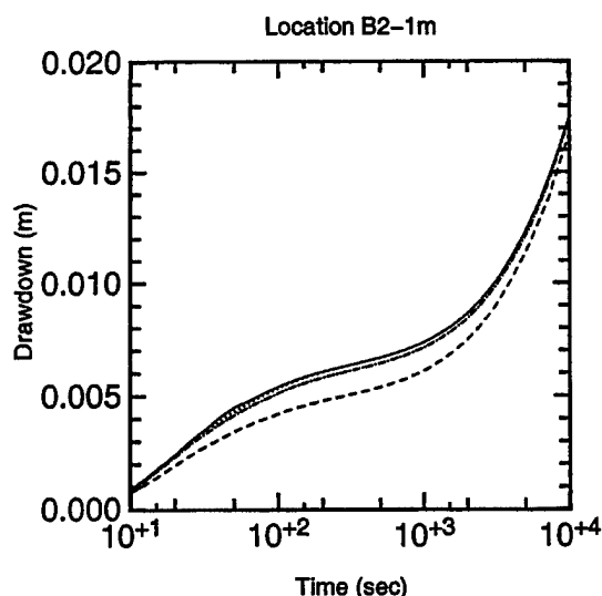
Figure 10: Comparison of drawdown at a depth of 1 m below the water table 3.52 m away from the well. WTAQ (solid), unmodified with 21 layers (dashed), unmodified with 26 layers (dot-dash), and modified with 21 layers (dotted).
