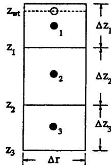
Figure 8: Cells with water table.
