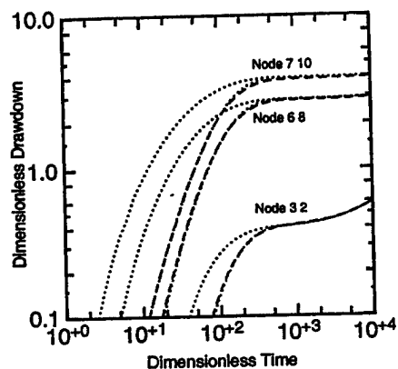
Figure 3: Comparison of cylindrical geometry model (dashed) to WTAQ calculations (solid).
