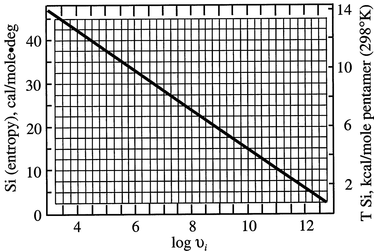
Figure 15: Plot of the above equation for entropy as a function of log(oscillator frequency) using the partition function of an harmonic oscillator. On the left-hand ordinate is plotted the entropy in cal/mol-deg (EU, entropy units), and on the right-hand ordinate is plotted the Gibbs free energy in kcal/mol at 298°K. This illustrates the increasing contribution of low frequency oscillations to the entropy of a polypeptide chain.
