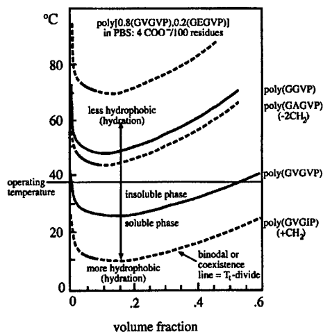
Fig. 2. Schematic representation of phase diagrams for several model elastic proteins based on the elastin repeat, (GVGVP)_n (see text for discussion). Solid curves adapted with permission from Sciortino et al. (1990) and (1993).
