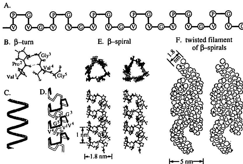
Fig. 3. Representations of the proposed molecular structure of (GVGVP)_n (see text for discussion).
