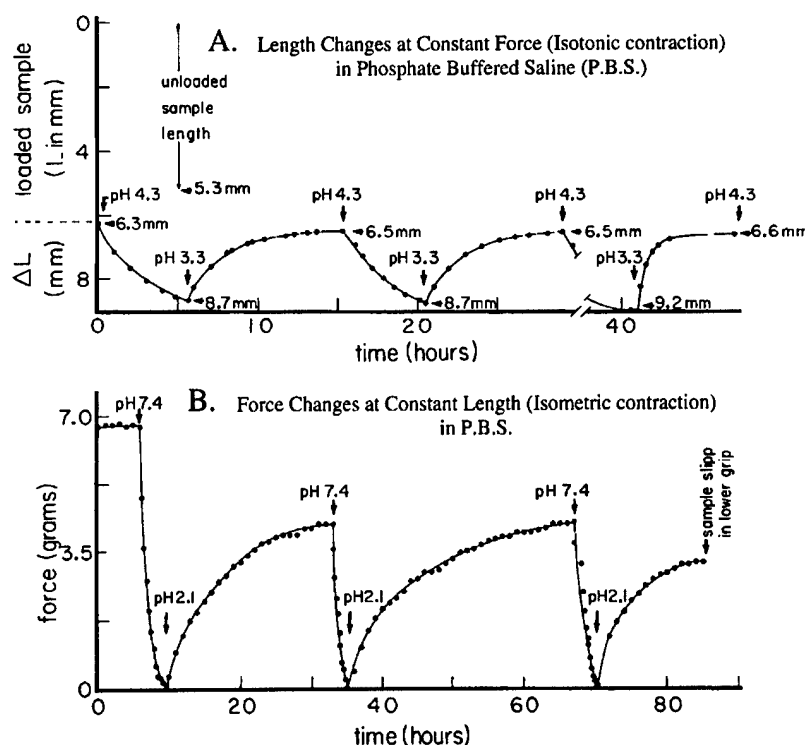
Fig. 9. Mechano-chemical coupling by 20 Mrad \gamma -irradiation cross-linked of poly[0.8(GVGVP),0.2(GEGVP)] under isotonic (A) and isometric (B) conditions. In part B under isometric contraction conditions there occurs an increase in entropic elastic force resulting from a decrease in entropy of the elastomer while there occurs an increase in the entropy of the solvent as hydrophobic hydration becomes bulk water. Therefore the increase in entropic elastic force cannot be the result of the solvent entropy change. Reproduced with permission from Urry et al. (1988b).
