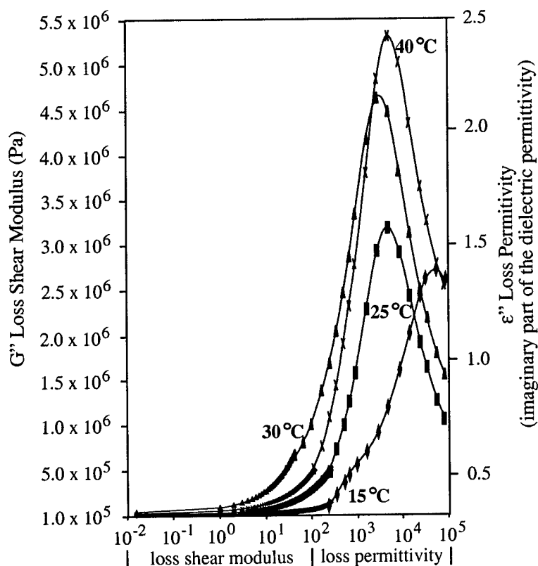
Figure 5: Melting of G'' and \epsilon'' data for (GVGIP)_{320}
