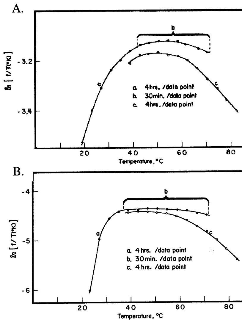
Figure 9: Thermoelasticity curves for A. fibrous elastin and B. 20 Mrad cross-linked poly(GVGVP). See text for discussion. Whether or not a near zero slope, i.e., an f_T/f \ll 1 , is obtained depends on the rate at which the temperature is raised. This is due to a slow denaturation at temperatures above 60°C. Reproduced with permission from Urry 1988a, 1988b.
