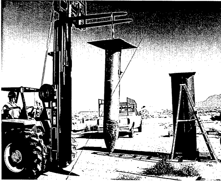
Figure G7. Penetrator on Support Plate/Cruise Cylinder
