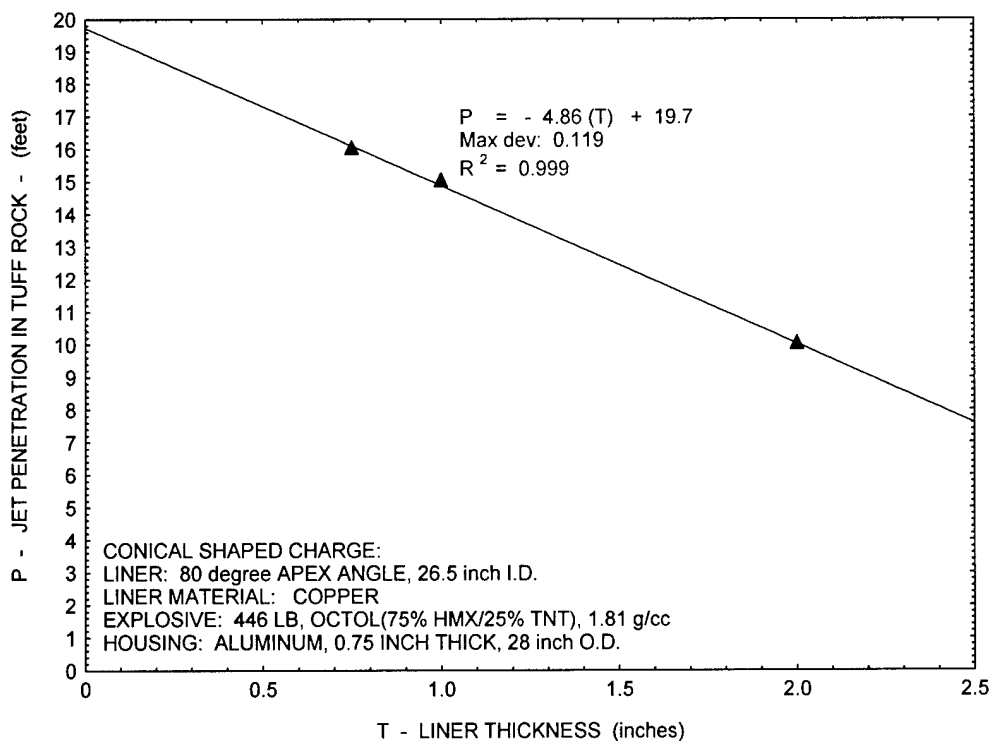
Figure C2. Jet Penetration Versus Liner Thickness
