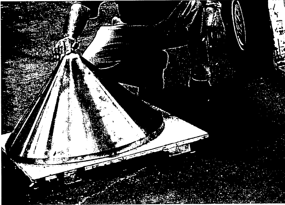
Figure 2. CSC Copper Cone/Explosive Side
