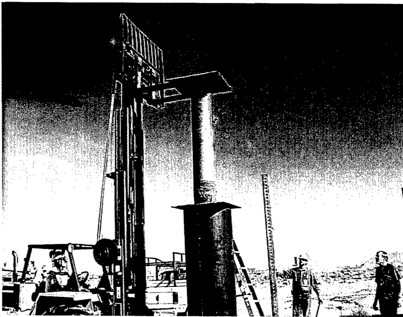
Figure G8. Penetrator Being Installed in Cruise Cylinder
