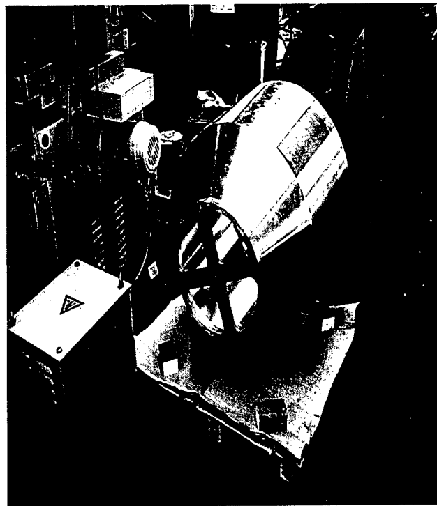
Figure B4. Aluminum Explosive Housing/Explosive Loading Fixture
