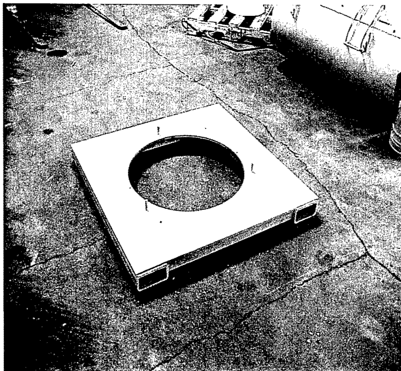
Figure 9. CSC Steel Support Platform (0.5 x 40 x 40 in. Al, 269.2 lb)
