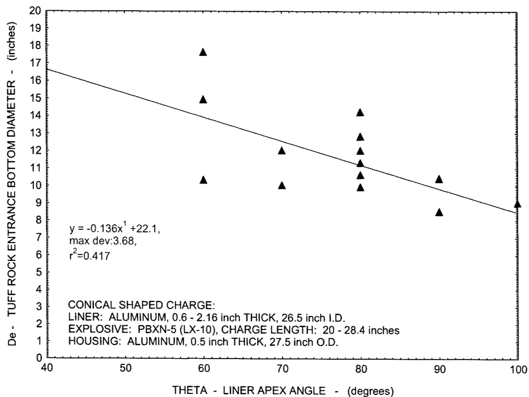
Figure C3. Entrance Hole Diameter Versus Liner Apex Angle
