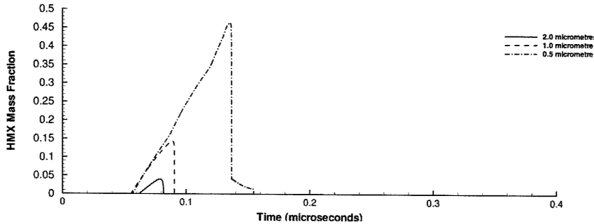
Figure 14: Comparison of pore collapse HMX mass fraction results. P_s = 2.2 GPa, \phi = 1.5\% and a_o = 0.5 - 2.0 \mu m .
