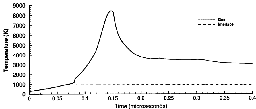
Figure 4: Viscoplastic pore collapse results for HMX - interface and gas temperature history. P_s = 2.2 \text{ GPa} , \phi = 0.5\% and a_o = 2.0 \mu\text{m} .
