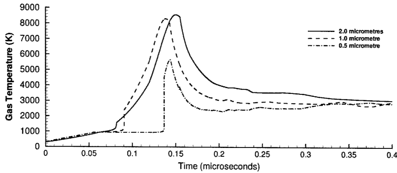
Figure 13: Comparison of pore collapse gas temperature results for HMX. P_s = 2.2 GPa, \phi = 1.5\% and a_o = 0.5 - 2.0 \mu m .
