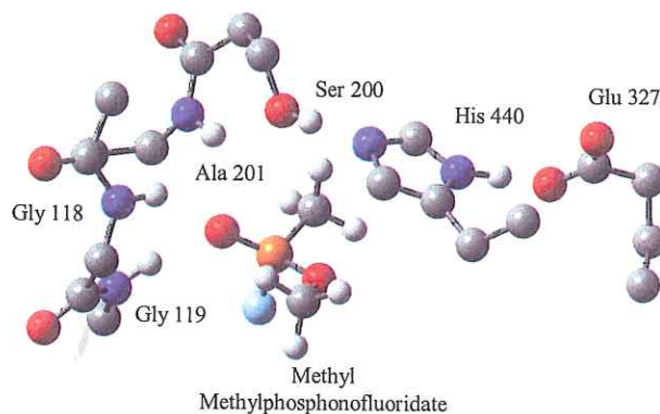
Figure 3. Significant residues of the active site of AChE ( Torpedo Californica ) with a generic OP compound, Methyl Methylphosphonofluoridate. For simplicity, only the significant protons are depicted. The catalytic triad consists of Ser-200, His-440, and Glu-327. The oxyanion hole consists of Gly-118, Gly-119, and Ala-201. The Ser-200 hydroxyl group is lined up opposite to the phosphinate fluoride. The phosphinyl group is coordinated in the oxyanion hole.
