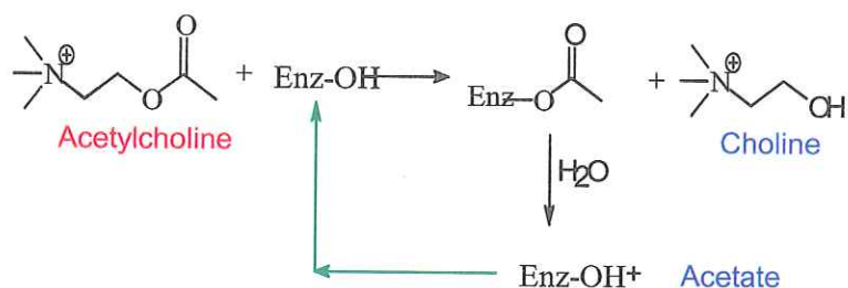
Figure 1. Schematic of the transesterification of acetylcholine and the regeneration of AChE via hydrolysis.
