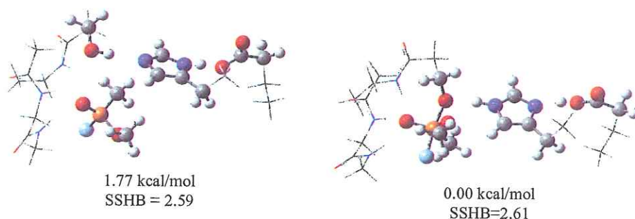
Figure 8. Reactant and product for the phosphonylation of the active site with the presence of the oxyanion hole (Gly-118, Gly-119 and Ala-201). QM/QM calculation using the ONIOM=(B3LYP/6-31G(d,p):B3LYP/STO-3G) levels of theory.
