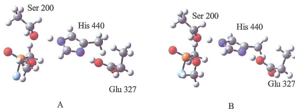
Figure 6. The TS's of the AChE ( Torpedo Californica ) catalytic triad reacting with Methyl Methylphosphonofluoridate at the A ) HF/6-31G(d) and B ) B3LYP/6-31G(d,p) levels of theory.
