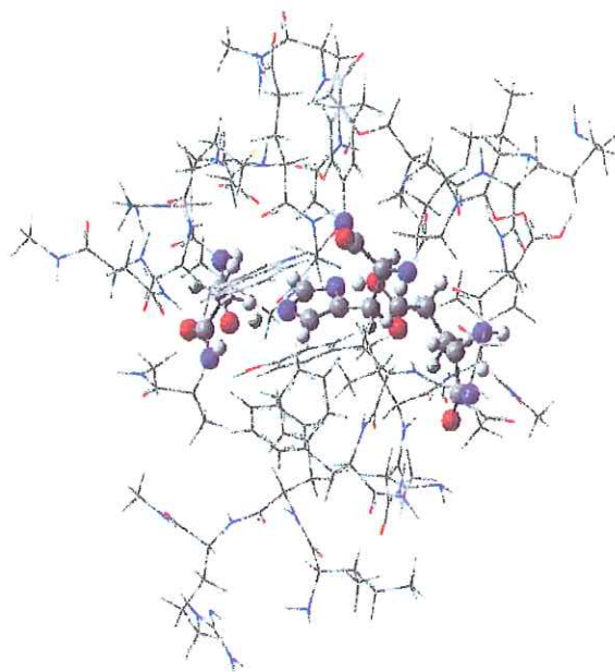
Figure 5. A 7Å AChE ( Mus Musculus ) example. The QM (Ball and stick) portion contains the catalytic triad residues calculated at the B3LYP/3-21G** level of theory. The MM (wire) portion, which surrounds the catalytic triad, is calculated using the UFF force field. Note the proper alignment of the catalytic triad. There are 254 heavy atoms plus 250 hydrogens in this example.
