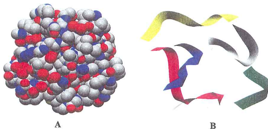
Figure 4. A) CPK model of a sphere of atoms with a radius of 10 angstroms from the Ser-200 hydroxyl group in the active site. B) The corresponding ribbon structure showing the five ribbon segments whose ends terminate on the sphere surface.
