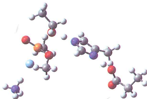
Figure 9. A QM B3LYP/6-31G(d,p) TS with the removal of fluoride via the participation of an ammonium ion.
