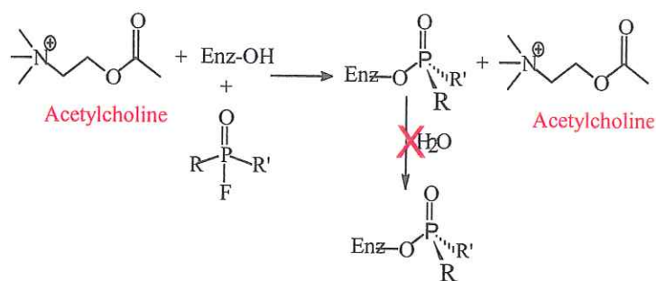
Figure 2. Schematic of the phosphorylation of AChE and the subsequent accumulation of acetylcholine.
