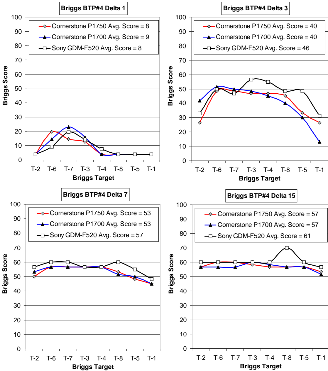
Figure II.21-3. Briggs Scores averaged for three NIDL observers for Delta-1, Delta-3, Delta-7 and Delta-15 contrast ratios on BPT#4 Test Patterns for the Cornerstone p1750 22-inch flat face Trinitron-type CRT monitor compared to the Cornerstone P1700 21-inch curved face shadowmask CRT monitor and compared to the Sony GDM-F520 flat face CRT monitor.
