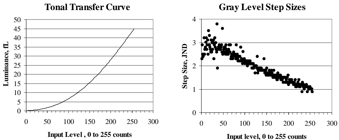
Figure II.6-1. System Tonal Transfer and perceptibility of gray level step sizes in Just Noticeable Differences (JNDs) for input counts 0 to 255 with front panel contrast control set to maximum.
