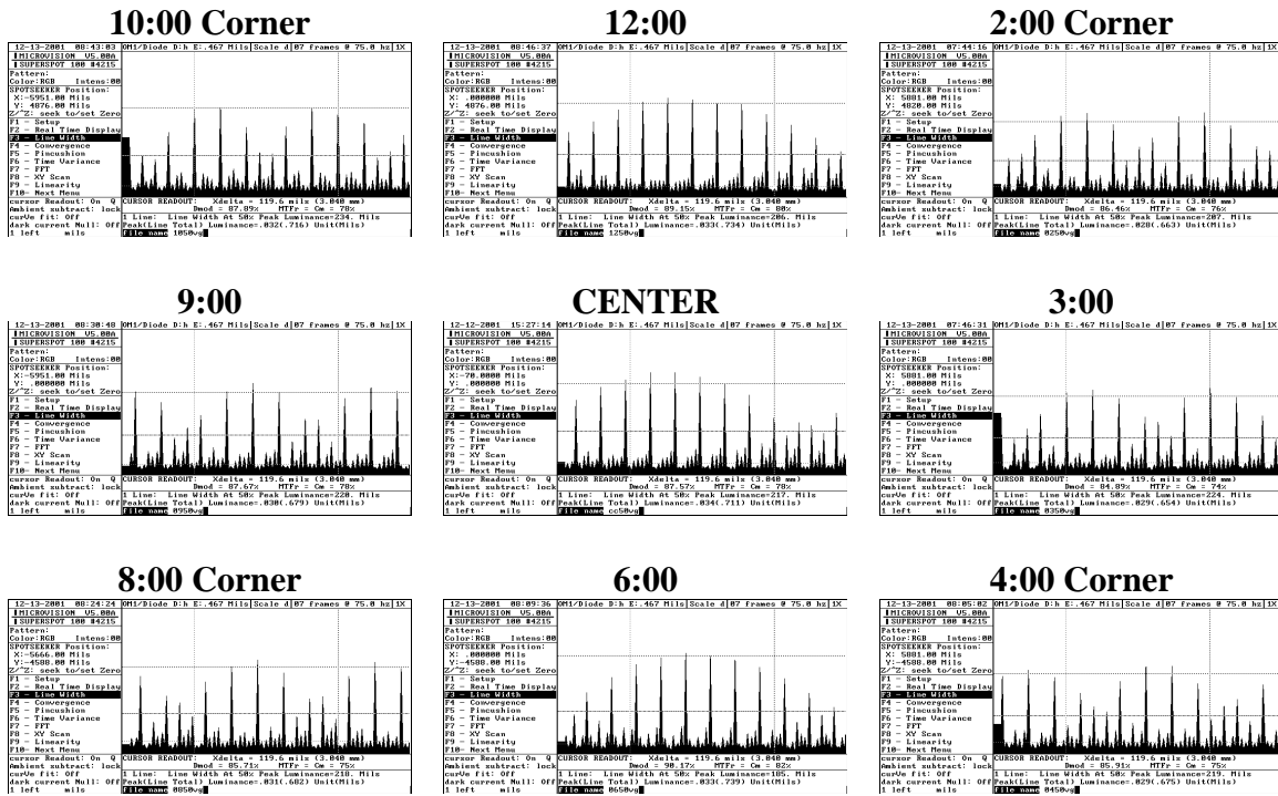
Figure II.12-2. Measured luminance profiles for horizontal and vertical grille patterns (1 pixel at input level corresponding to 50% Lmax, 1 pixel at level 0 = Lmin) for the Cornerstone p1750 monitor. V-grilles exhibit extensive moiré due to aliasing.
