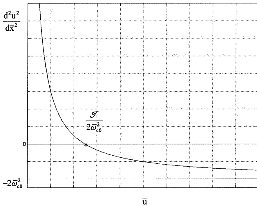
Figure 12 Following (2.48): the second derivative d^2 \bar{u}^2 / dx^2 as a function of \bar{u} .
