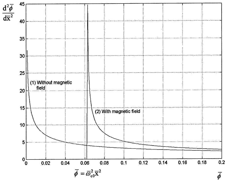
Figure 4 Poisson equation without (1) and with (2) the magnetic field B expressed in terms of \bar{\omega}_{c0} .
