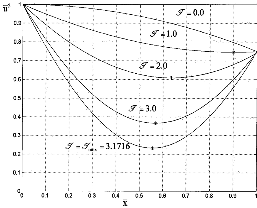
Figure 11a The dependence of the velocity function \bar{u}^2(\bar{x}) on the injection current \iota for \bar{\omega}_{c0} = 0.5 .
