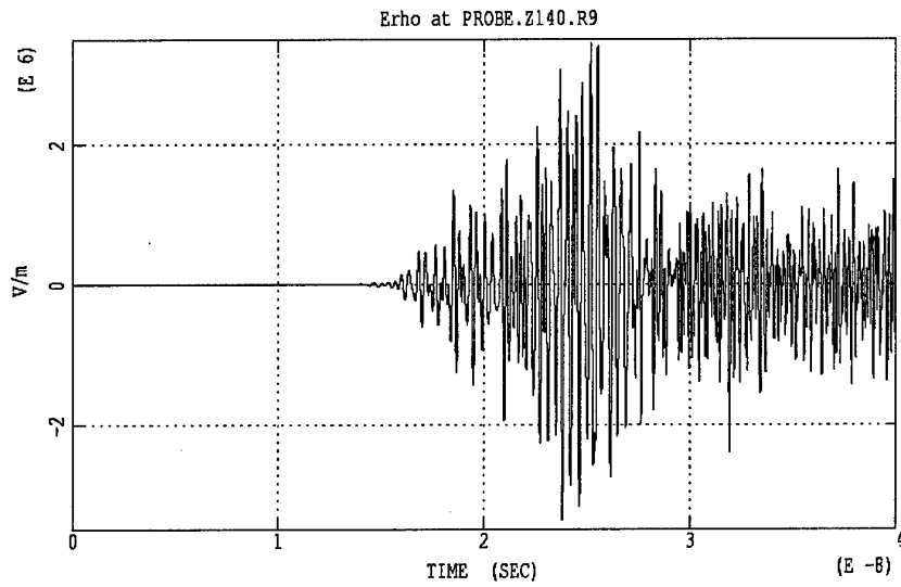
Figure 3a E_p field intensity as recorded near the output window.
