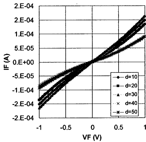
a) Non-linear I-V profiles of the TLM structures
