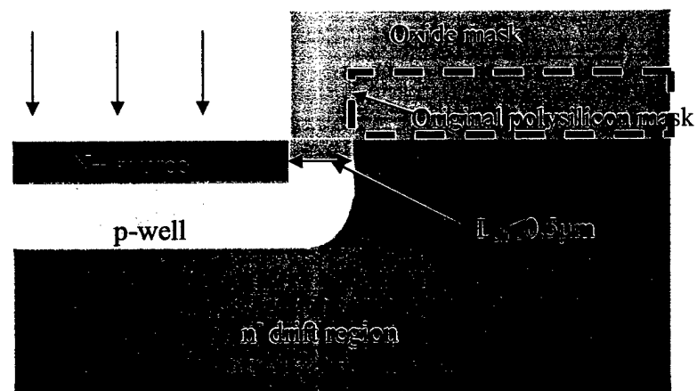
c) Source implantation
