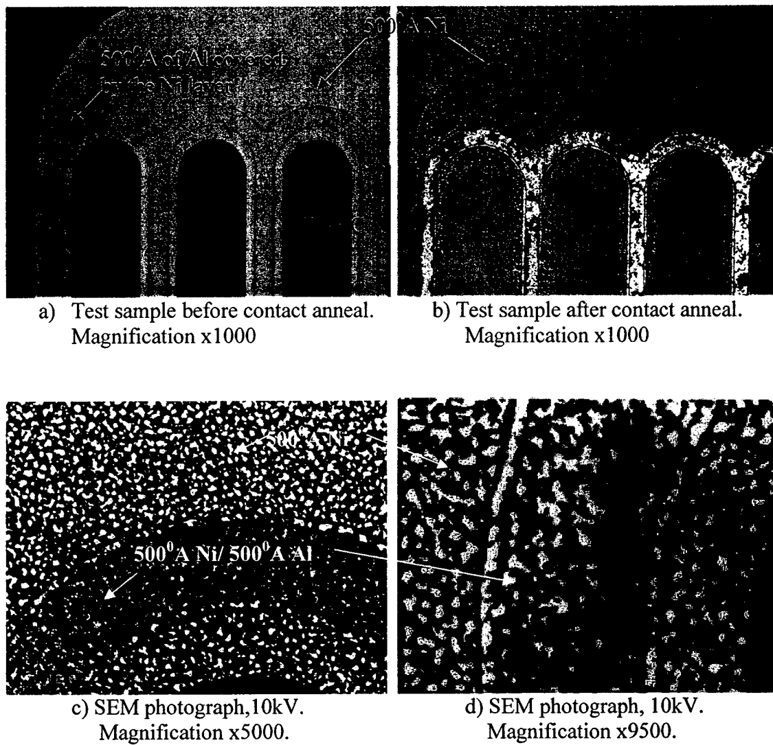
Fig. 8.22. Contact anneal experiment performed on 6H-SiC test piece before annealing the 4H-50 \mu m sample at 900 ^{\circ} C in 400mT Ar pressure for 2 minutes.
