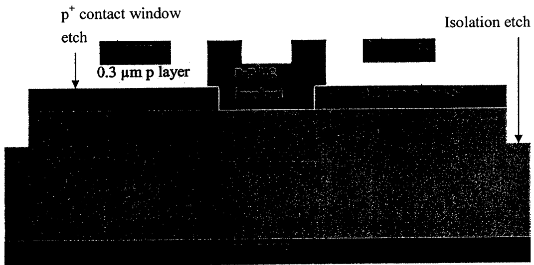
g) After RIE of isolation etch
