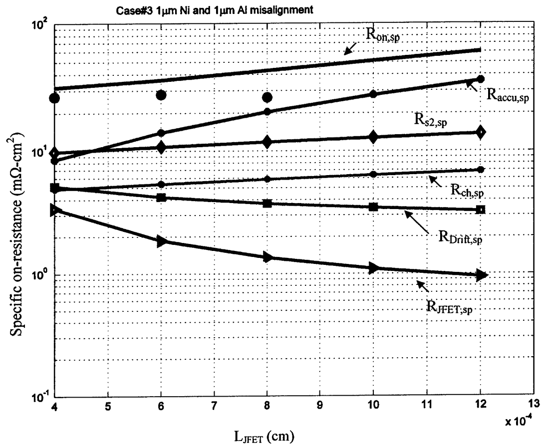
Fig.8.19. Specific on-resistance of the 0.5 \mu m channel length DMOSFETs on the 4H-20 \mu m sample for 2-3 design rules, assuming 1 \mu m misalignment of the Ni contacts and 1 \mu m misalignment of the Al contacts . The circles are the measured data and the solid lines are the specific on-resistances from spreadsheet calculations.
