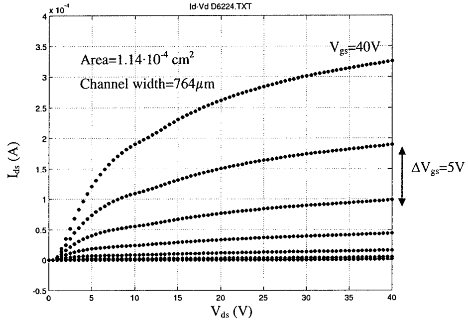
b) I-V characteristics of a device in 4H-SiC on a 50 \mu\text{m} epilayer
