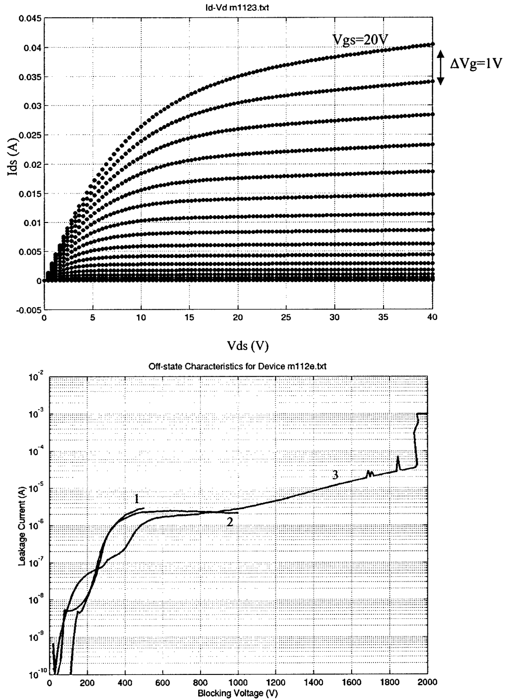
Fig. 8.2 Forward and reverse characteristics of a DMOSFET on 4H-20 \mu m with L_{JFET}=6\mu m and A=1.144 \cdot 10^{-4} \text{ cm}^2 with 2-3 design rules. Curves 1, 2, and 3 represent repeated high voltage measurements on the same device.
