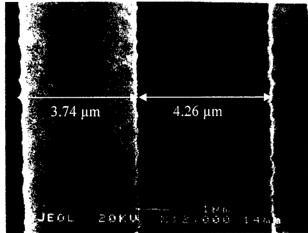
b) SEM picture of alignment marks before oxidation.
