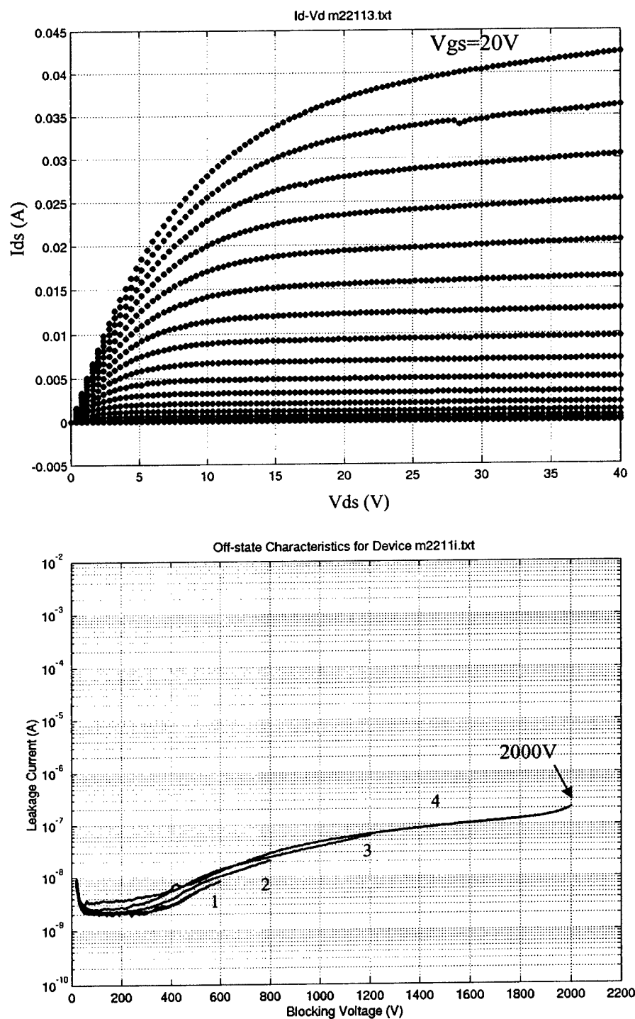
Fig. 8.5. Forward and reverse I-V characteristics of a DMOSFET on 4H-20 \mu m sample with 3-5 design rules, L_{JFET}=6\mu m and A=1.56\cdot 10^{-4} cm 2 . Curves 1, 2, 3, and 4 represent repeated high voltage measurements on the same device during the off-state.
