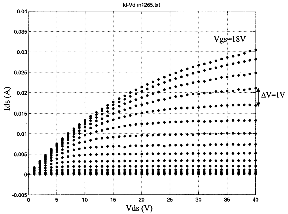
Fig. 8.26c. Forward drain characteristics of a DMOSFET on the 4H-50 \mu m sample with 2-3 design rules, L_{JFET}=8\mu m and A=1.248 \cdot 10^{-4} \text{ cm}^2 .
