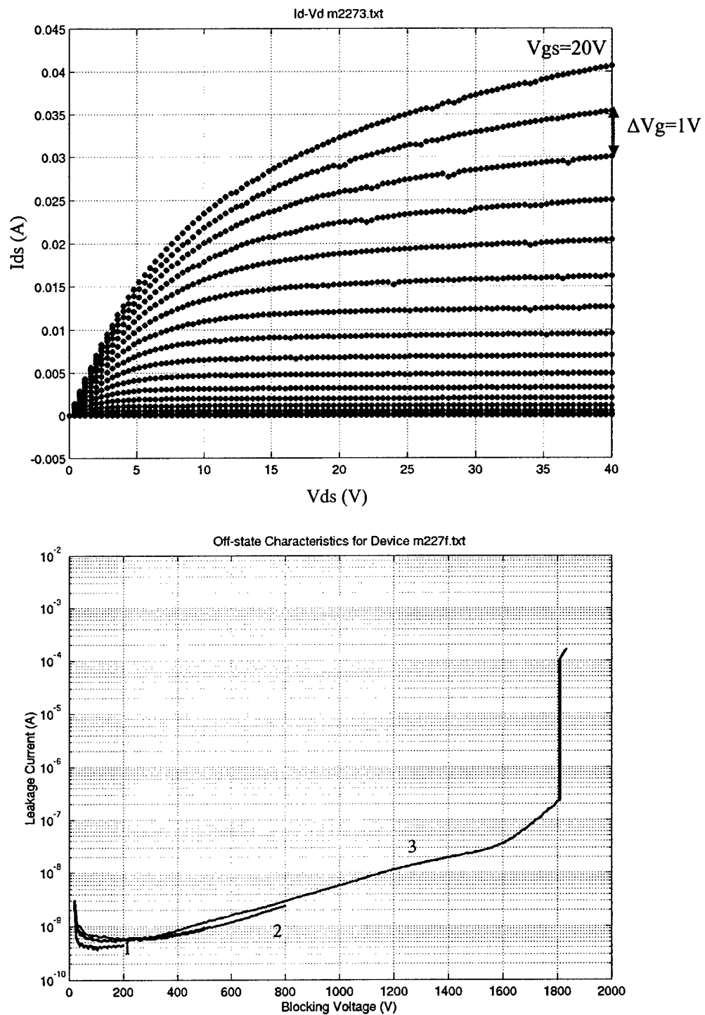
Fig. 8.4. Forward and reverse I-V characteristics of a DMOSFET on 4H-20 \mu\text{m} sample with 3-5 design rules L_{JFET} = 4 \mu\text{m} and A = 1.456 \cdot 10^{-4} \text{ cm}^2 . Curves 1, 2, and 3 represent repeated high voltage measurements on the same device during the off-state.
