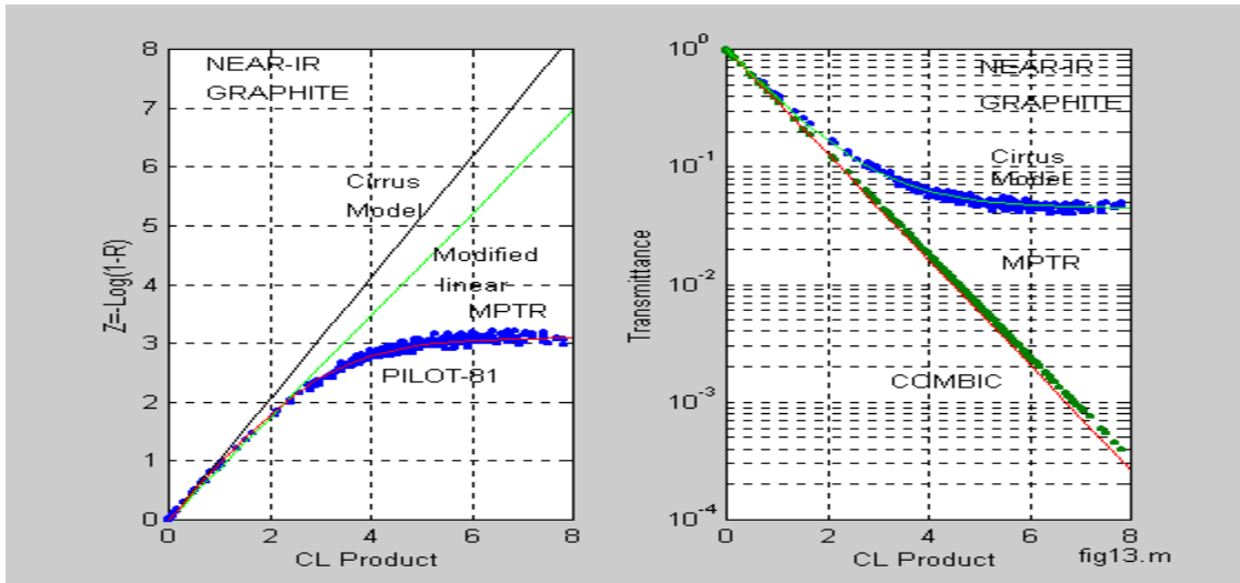
Figure 12. Example comparing linear models with theory.
