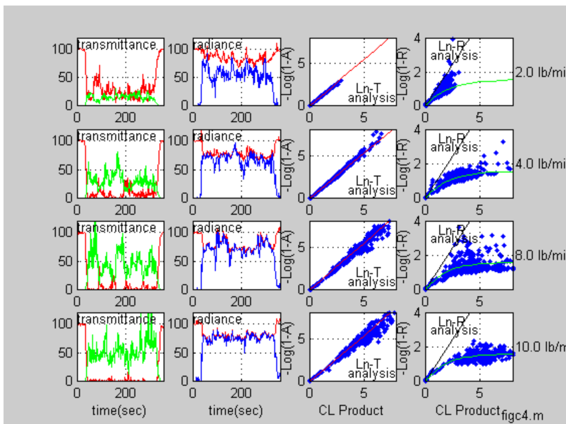
Figure C4. Multi-trial summary, brass mid-ir.
