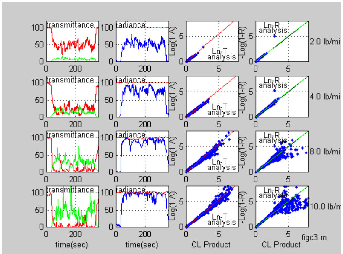
Figure C3. Multi-trial summary, brass-visible.
