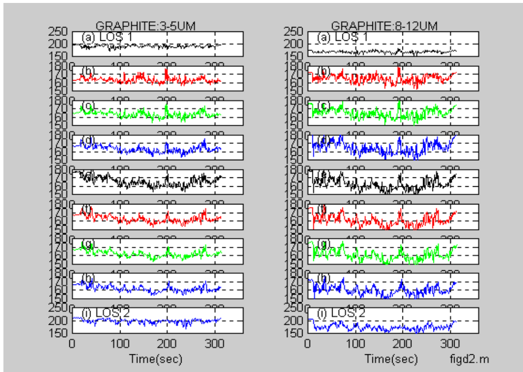
Figure D2. Dual band multi-pixel time scans of total radiance for graphite.
