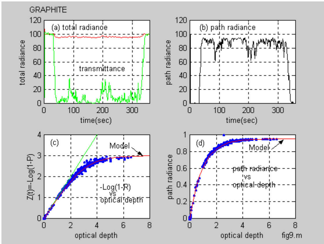
Figure 8. Demonstration of Log-R correlation method applied to MPTR radiometer data.
