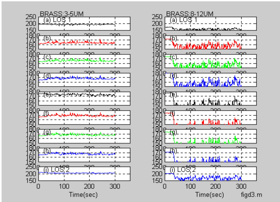
Figure D3. Dual band multi-pixel time scans of total radiance for brass.
