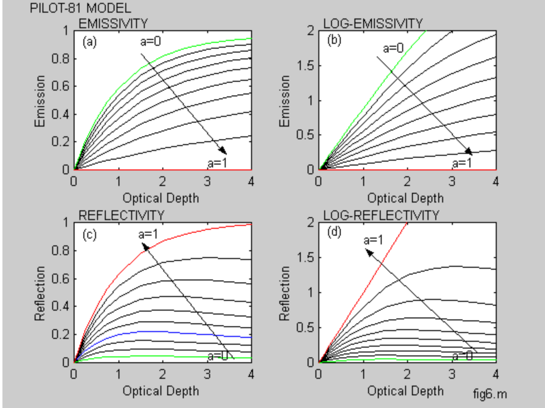
Figure 6. Theoretical calculations of emissivity and reflectivity ( I ).
