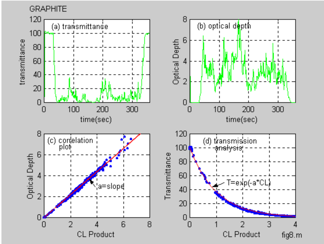
Figure 7. Demonstration of the Log T correlation method applied to the MPTR transmissometer data.
