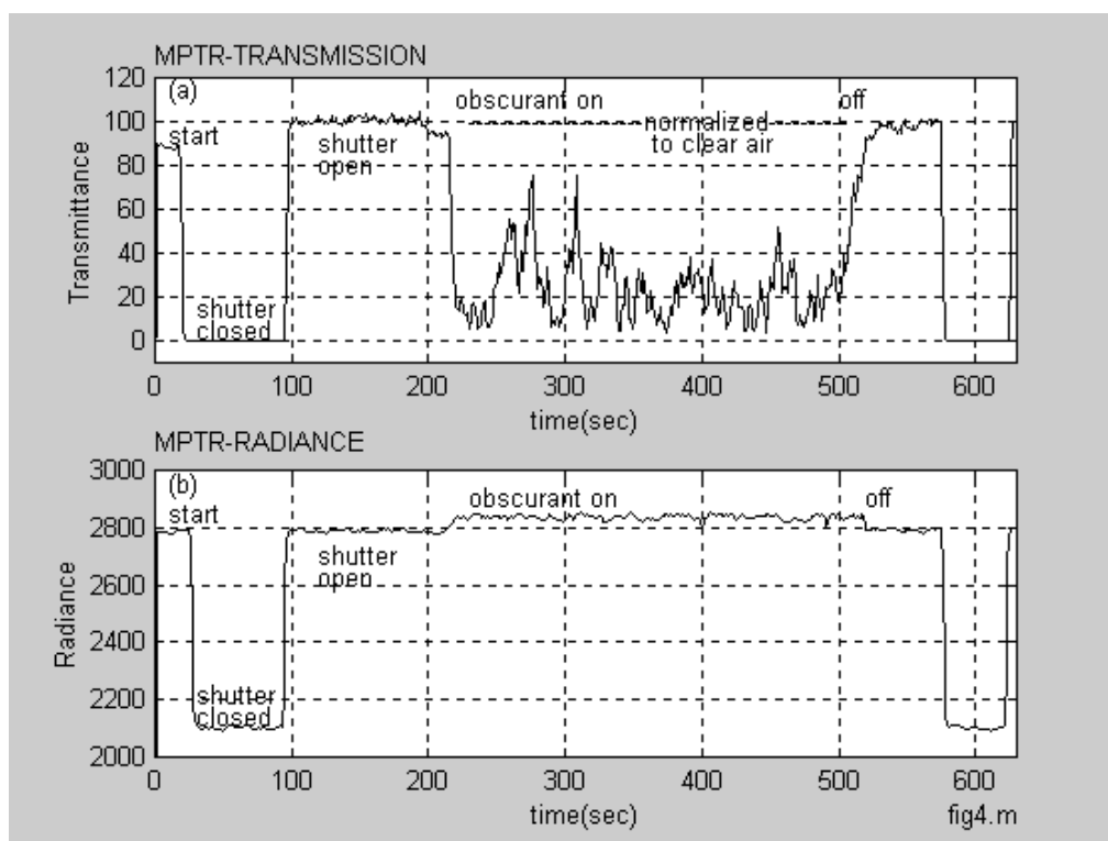
Figure 4. Examples of MPTR signals for (a) transmissometer mode and (b) radiometer mode.
