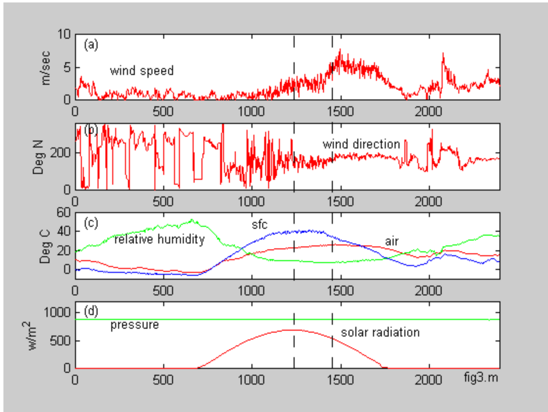
Figure 3. On site meteorological measurements.
