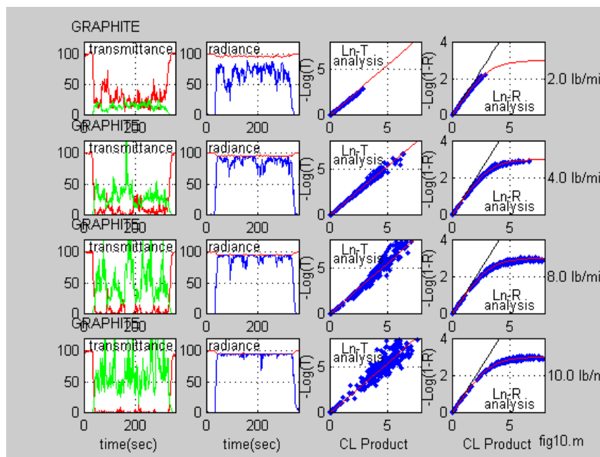
Figure 9. Example of multi-trial analysis for graphite, near IR.
