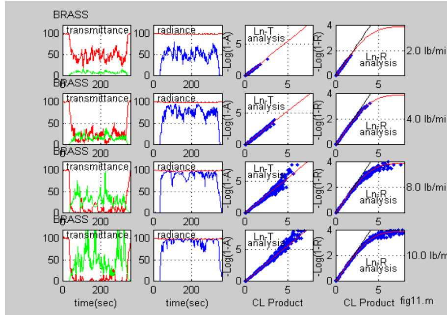
Figure 10. Example of multi-trial analysis for brass, near IR.
