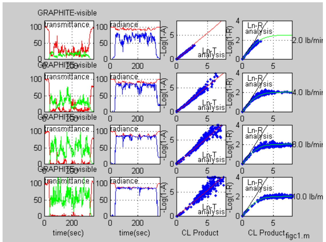
Figure C1. Multi-trial summary, graphite-visible.
