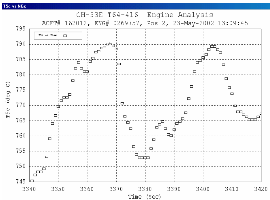
Figure 6-1-6. Temperature vs. Time, CH-53E
