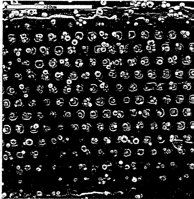
Figure 3: Wax Substrate With 1µm Copper Particles
