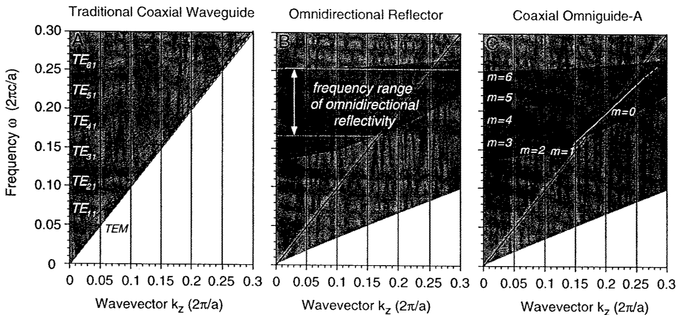
Fig. 2. Projected band structures along an axial direction. (A) Traditional metallic coaxial cable with inner and outer coaxial radii of r_i = 3.00 a and r_o = 4.67 a , respectively. The red bands correspond to allowed guided modes. For any given wavevector, the lowest frequency mode is a TEM mode characterized by a perfectly linear dispersion relation. The six next highest bands correspond to transverse electric ( TE_{ml} ) modes with l = 1 and increasing angular momentum m . (B) Omnidirectional, reflecting, all-dielectric multilayer film. Light-blue regions correspond to modes for which light is allowed to propagate within the dielectric mirror, and dark-blue regions correspond to modes for which light is forbidden to propagate within the dielectric mirror. The diagonal black line identifies
