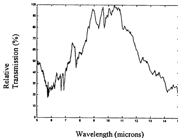
Fig. 4. Transmission through the hollow waveguide around a 90^\circ bend as a function of wavelength.
