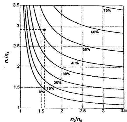
Fig. 3. (left) The range to midrange ratio (\omega_h - \omega_l)/1/2(\omega_h + \omega_l) , for the fundamental frequency range of omnidirectional reflection, plotted as contours. Here, the layers were set to quarter wave thickness and n_1 > n_2 . The ratio for our materials is about 45% ( n_1/n_2 = 2.875 and n_2/n_0 = 1.6 ). It is located at the intersection of the dashed lines (black dot).
