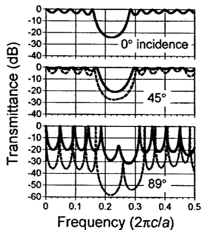
Fig. 3. Calculated transmission spectra for a quarter-wave stack of ten films ( n_1 = 1.7, n_2 = 3.4 ) for three angles of incidence. Solid curves, p -polarized waves; dashed curves, s -polarized waves. The overlapping region of high reflectance ( >20 dB) corresponds to the region between the open and filled circles of Fig. 2.
