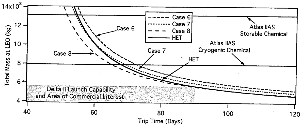
Fig. 3. Mass at LEO for hydrogen arcjet-neutralizer (Cases 6-8) for various trip times.
