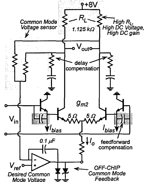
Figure 5: Integrator Design
