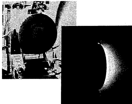
Figure 16: Aerojet MSAT 50 kW Hall Thruster
