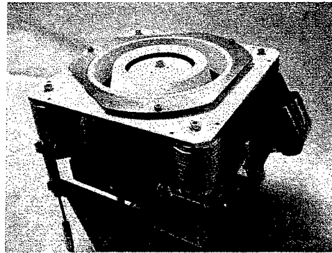
Figure 18: Snecma PPS ® X000 Development Model
