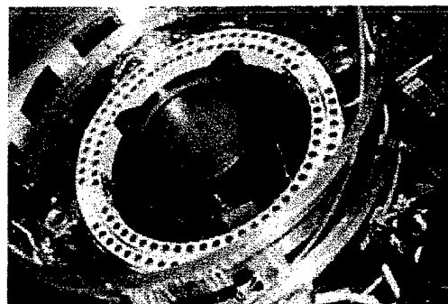
Figure 21: NSTAR Ion Engine Mounted on Deep Space 1
