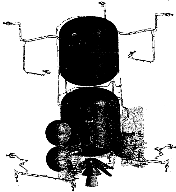
Figure 1: Typical Unified Propulsion Design Layout
