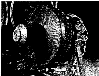
Figure 29: Mark V Pulsed Inductive Thruster
