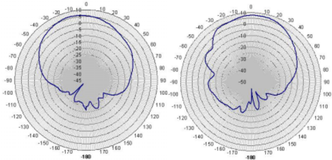
Figure 20. The VPOL Free-space Radiation Patterns of the Receiving Antenna ( \Phi = 0^\circ ) and the Transmitting Antenna ( \Phi = 180^\circ ) on NPSAT-1
