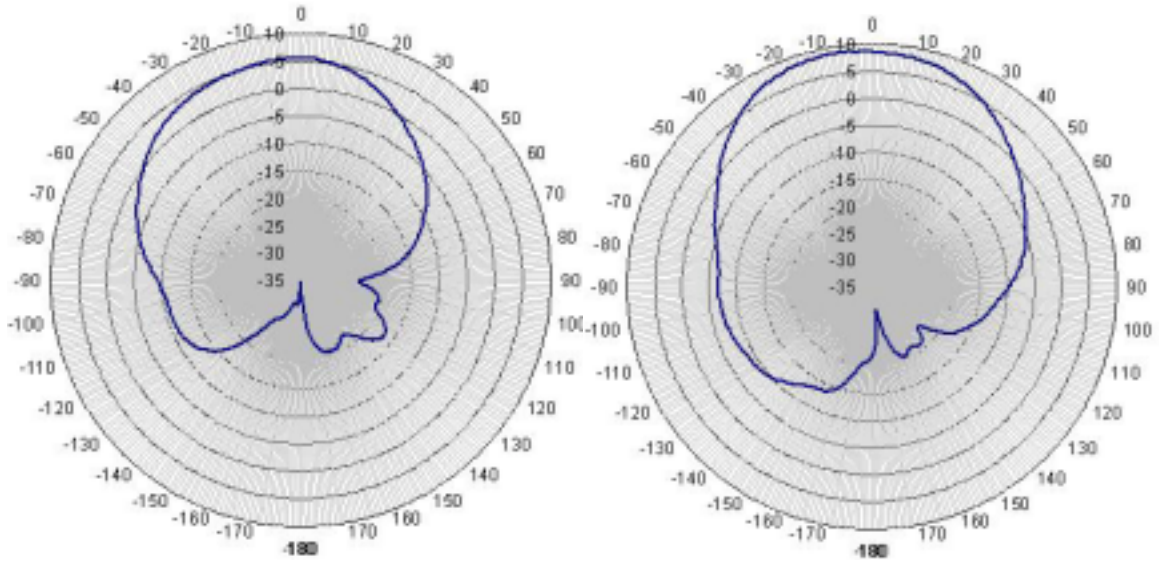
Figure 11. The VPOL Free-space Radiation Patterns of the Receiving Antenna ( \Phi = 90^\circ ) and the Transmitting Antenna ( \Phi = -90^\circ )
