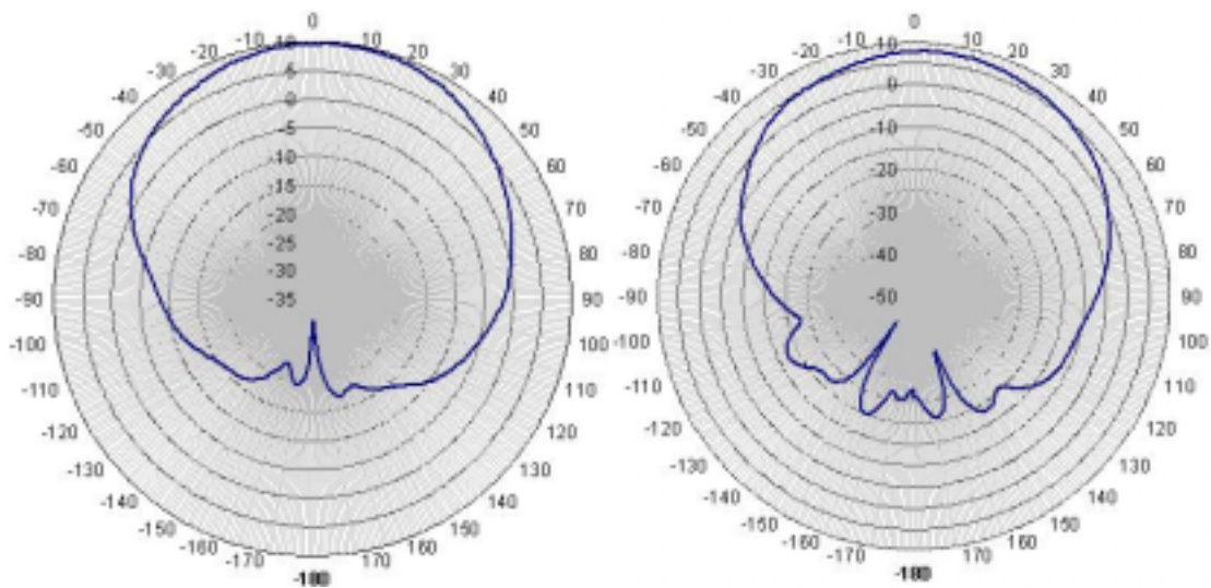
Figure 17. The HPOL Free-space Radiation Patterns of the Receiving Antenna ( \Phi = 0^\circ ) and the Transmitting Antenna ( \Phi = 180^\circ )
