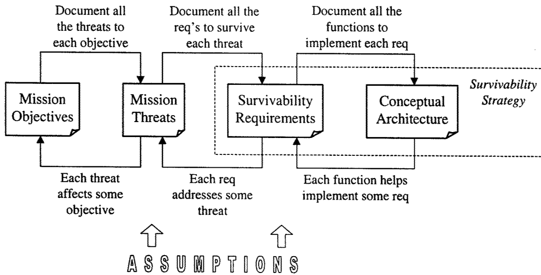
Figure 8: Survivability Tracing from Mission to Conceptual Architecture
