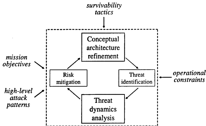
Figure 10: Survivability Strategy Refinement Process
