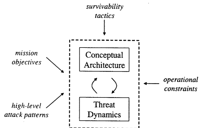
Figure 4: Survivability Strategy Refinement Process Overview
