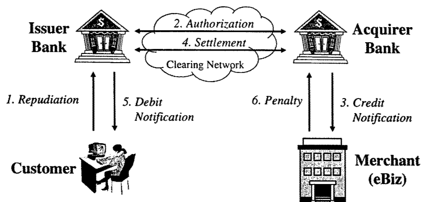
Figure 17: Online Credit Card Payment Repudiation
