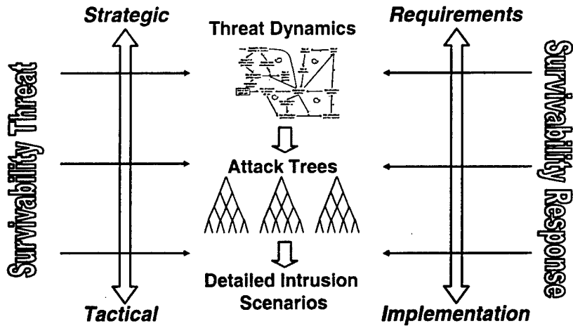
Figure 7: Structured Intrusion Analysis
