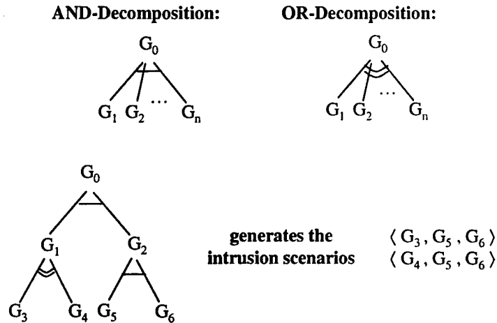
Figure 6: Attack Tree Representation
