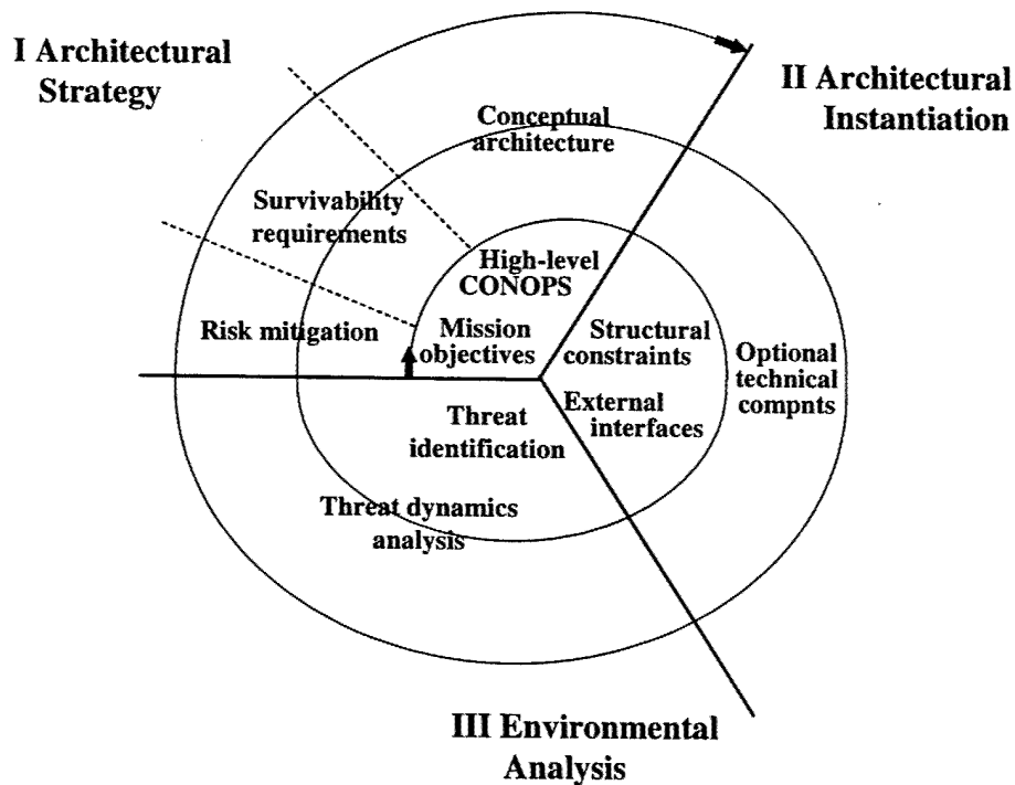
Figure 14: eBiz Survivability Strategy Development Process
