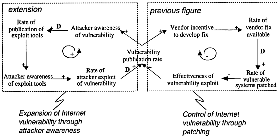
Figure 13: The Effects of Vulnerability Publication on Internet Vulnerability
