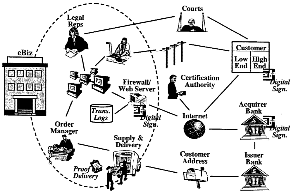
Figure 24: Final eBiz Conceptual Architecture
