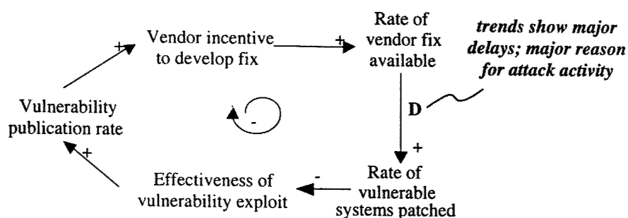
Figure 12: A Feedback Loop for Controlling Vulnerability
