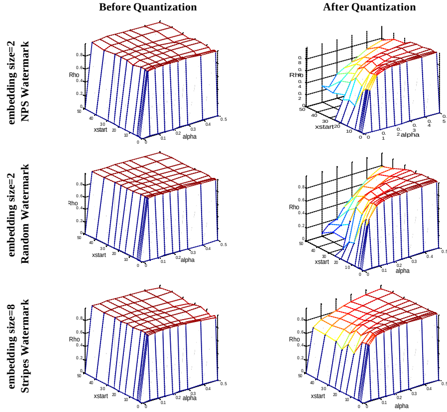
Figure 23. Mean r Achieved by Synthetic Images for Various Embedding Sizes and Watermarks.
