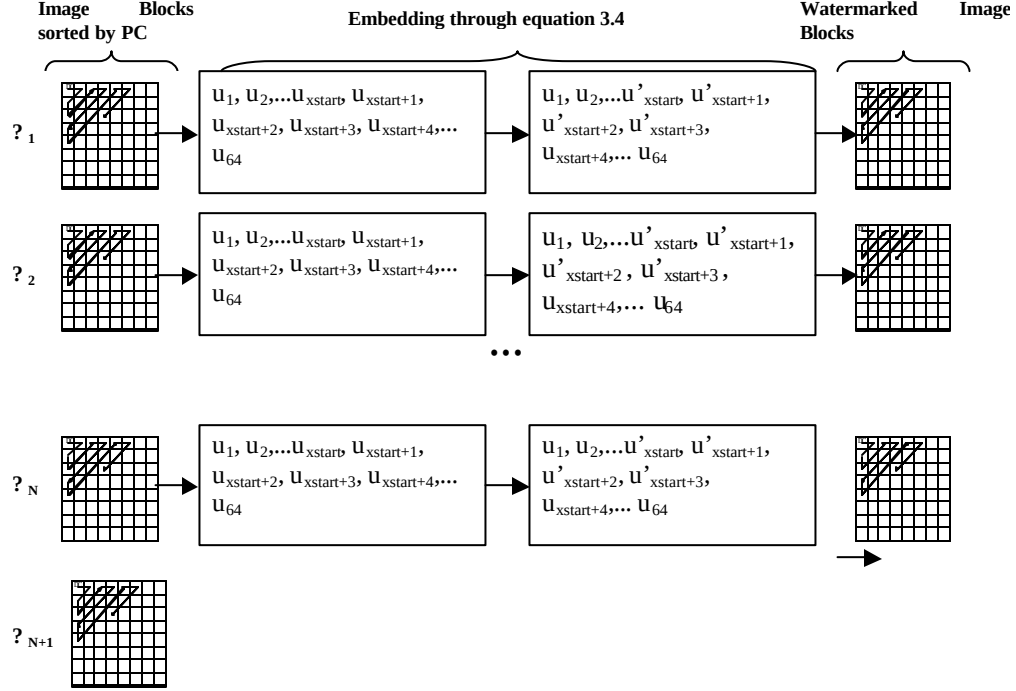
Figure 11. The Embedding Process.
