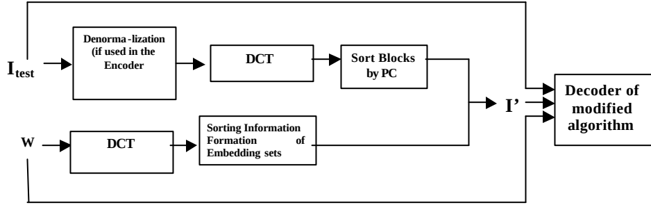
Figure 36. Decoder for the Second Semi-Blind Variation.
