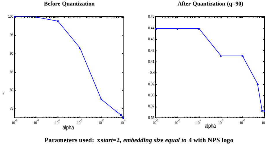
Figure 37. Comparison of the PC Sorting of Original and Marked Images.
